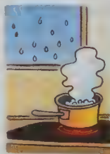
condensation
