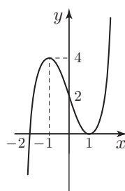
y = x^3 - 3x + 2 figure 3
