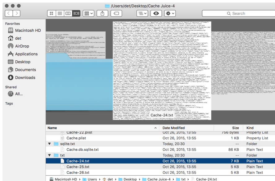
Figure 10-4: Examining the contents of the cache databases, split into separate files and directories by File Juicer
