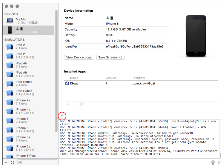
Figure 10-1: The Devices window in Xcode
