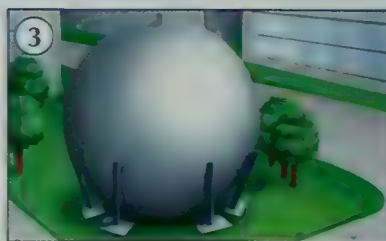
3. natural gas
