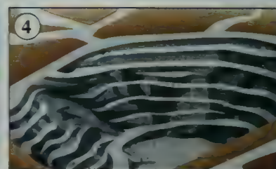
4. coal
