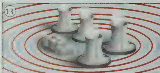
13. radiation
