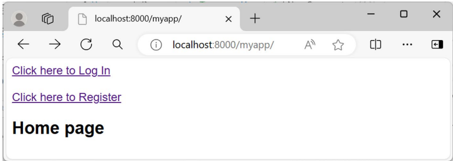
Figure 6-3. Home page
