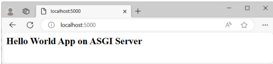
Figure 1-7. ASGI app
