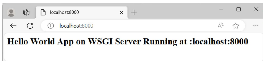
Figure 1-4. WSGI app
