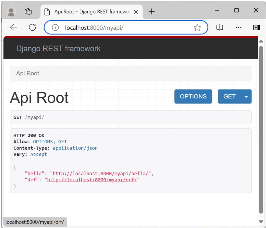
Figure 7-4. Api root
