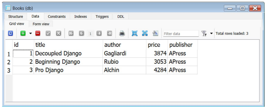
Figure 3-2. Books table
