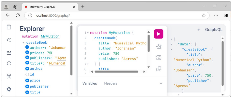
Figure 8-7. GraphiQL output of createBook mutation
