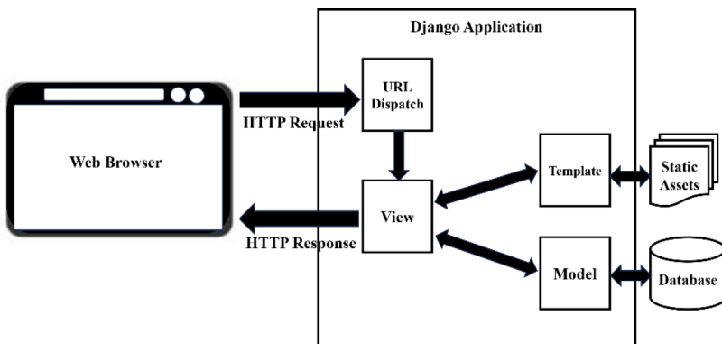
Figure 1-6. MVT pattern
