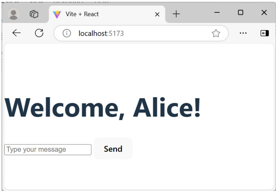
Figure 10-11. Chat interface
