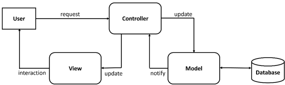
Figure 1-5. MVC architecture
