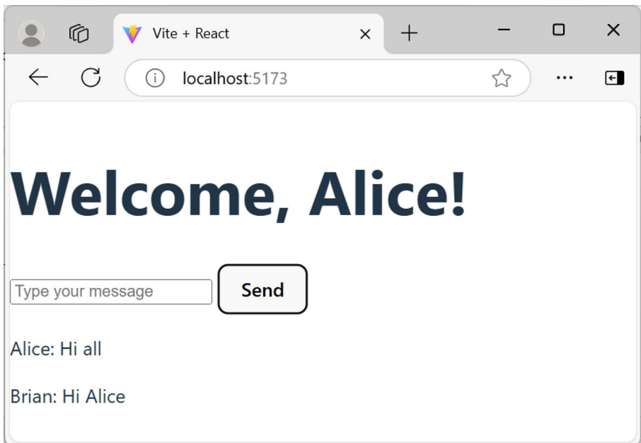
Figure 10-12. Chat log
