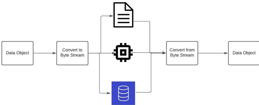
Figure 7-2. Object serialization
