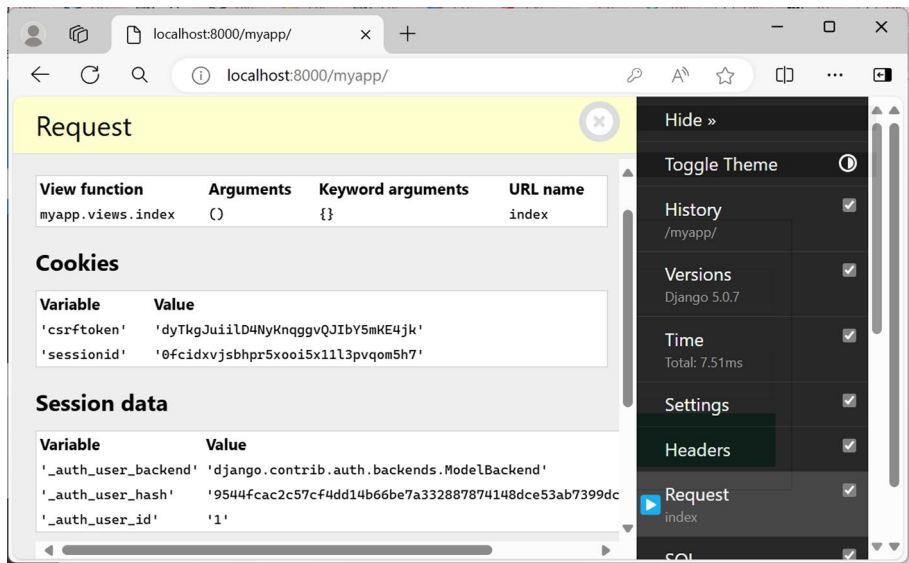
Figure 6-14. Request panel
