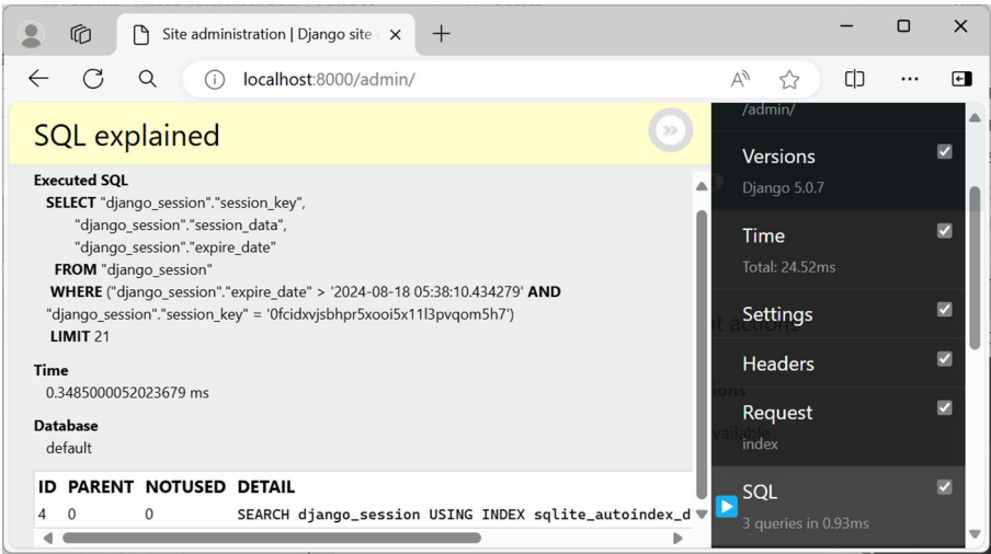
Figure 6-13. SQL explained
