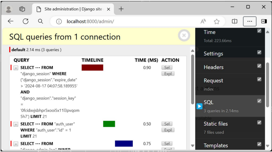
Figure 6-12. SQL panel
