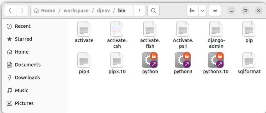
Figure 2-3. django-admin utility
