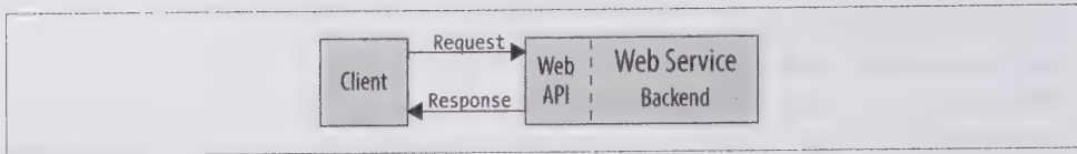
Figure 1-1. Web API
