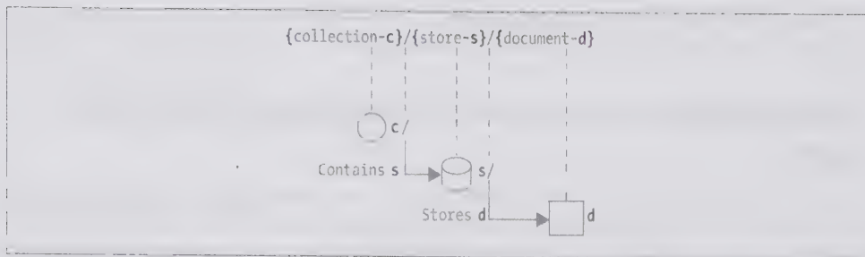
Figure 2-1. WRML diagram of a URI's associated resource model
