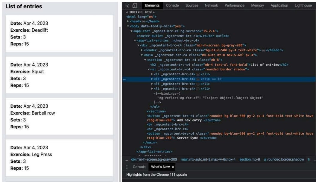
Figure 4.3 – Chrome DevTools
