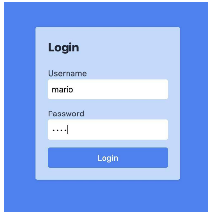
Figure 7.4 – Login page
