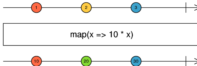
Figure 9.3 – Map operator marble graph (source: https://rxjs.dev/api/index/function/map , MIT license)
