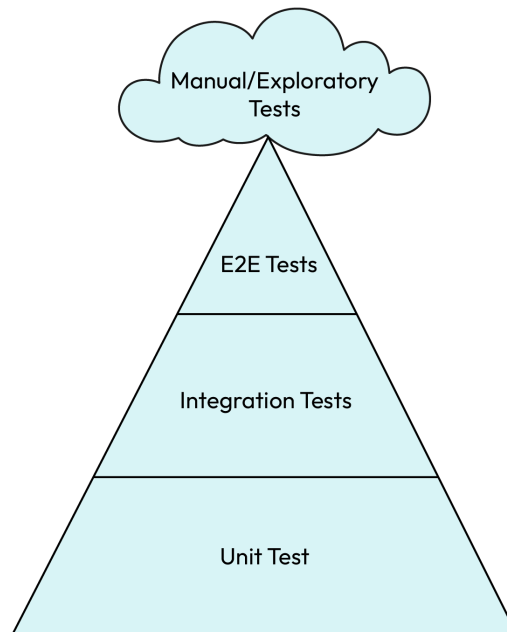
Figure 10.1 – Test pyramid
