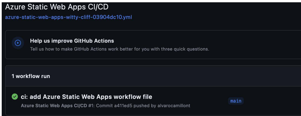
Figure 12.15 – GitHub action
