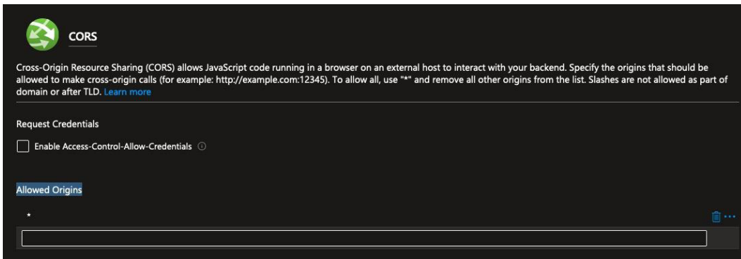
Figure 12.7 – CORS configuration
