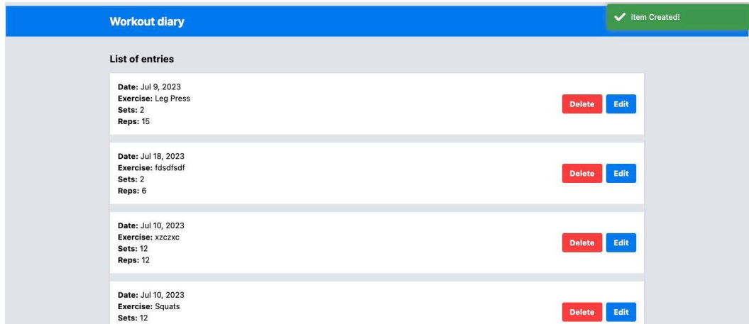
Figure 8.4 – Success notification
