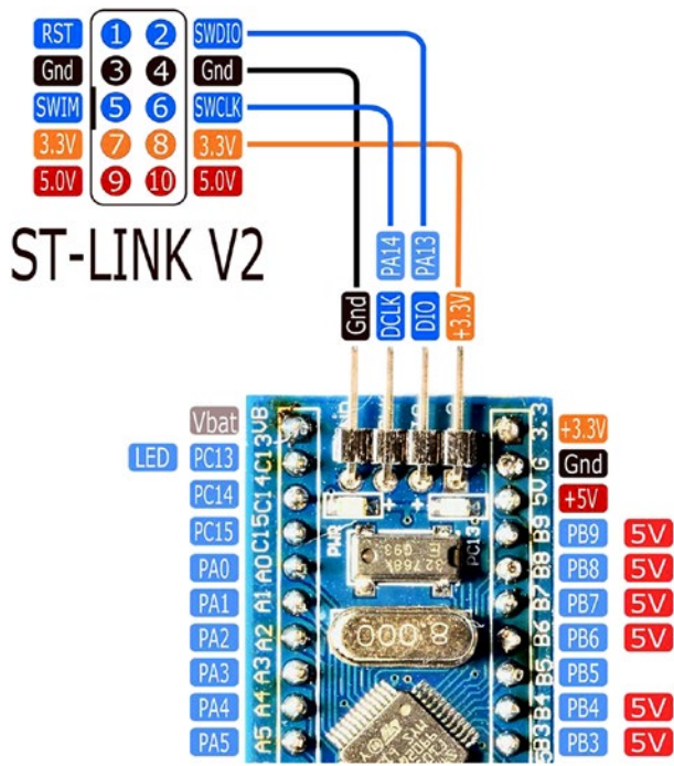
Figure 3-6. ST-Link V2 programmer hookup to the STM32F103C8T6 device. Check the connections on the device you have; assume ST-Link programmers are different.
