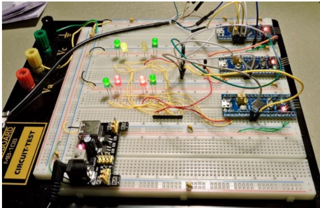
Figure 18-5. Breadboard setup of CAN demo
