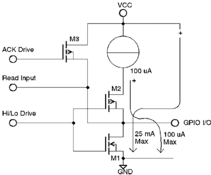
Figure 11-7. PCF8574 simplified GPIO circuit
