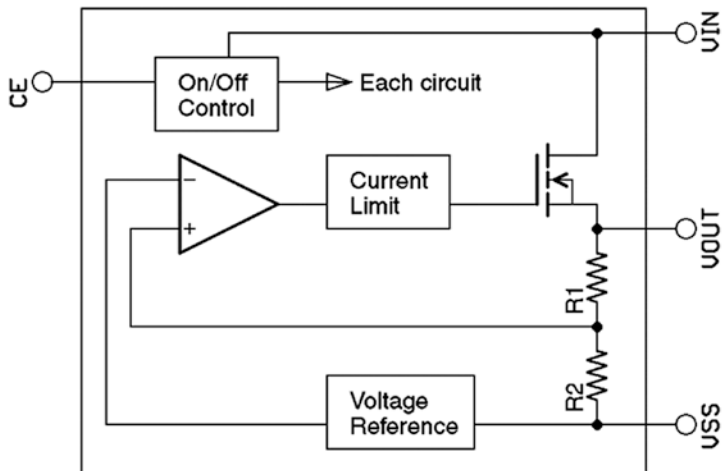
Figure 3-3. Block diagram of the 5- to 3.3-volt regulator
