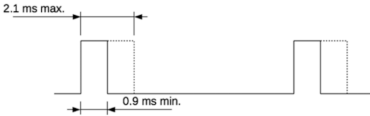
Figure 17-1. Typical RC servo signal
