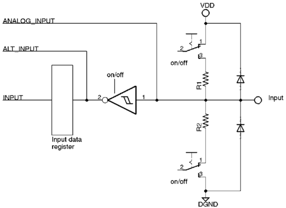
Figure 4-2. Basic structure of the GPIO input
