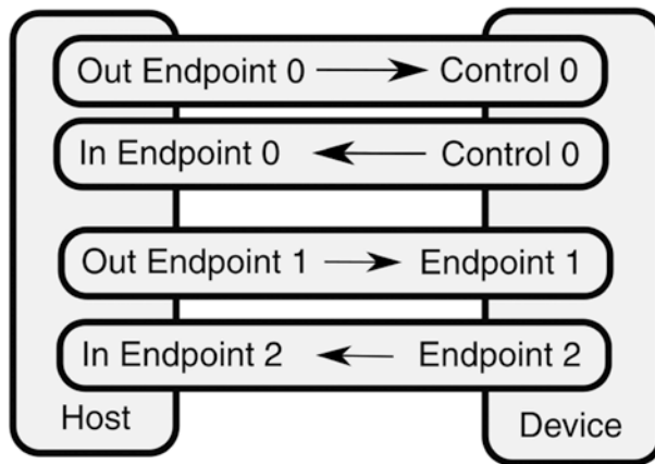
Figure 7-4. USB pipes and endpoints
