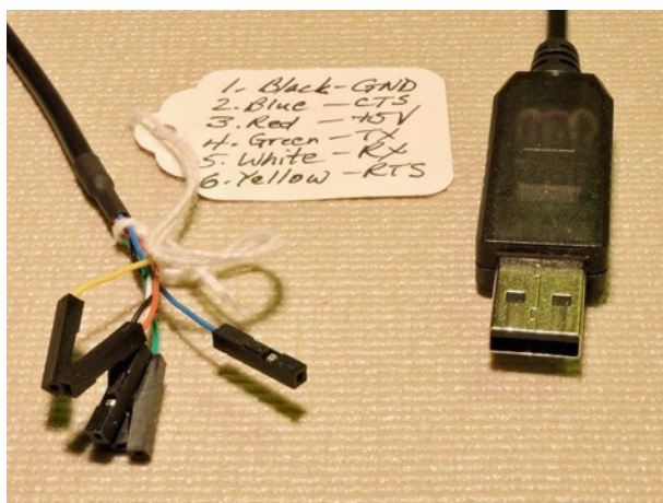
Figure 1-6. A USB-to-TTL serial (5V) adapter cable
