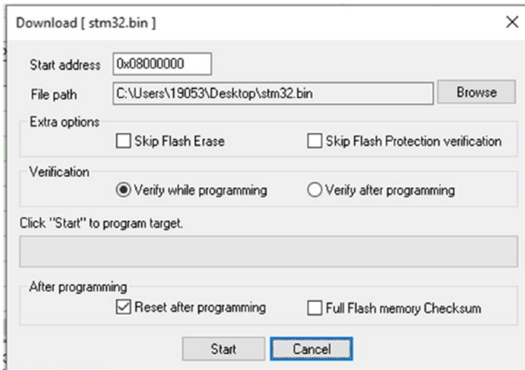
Figure 3-9. The Utility Target ► Program... dialog options
