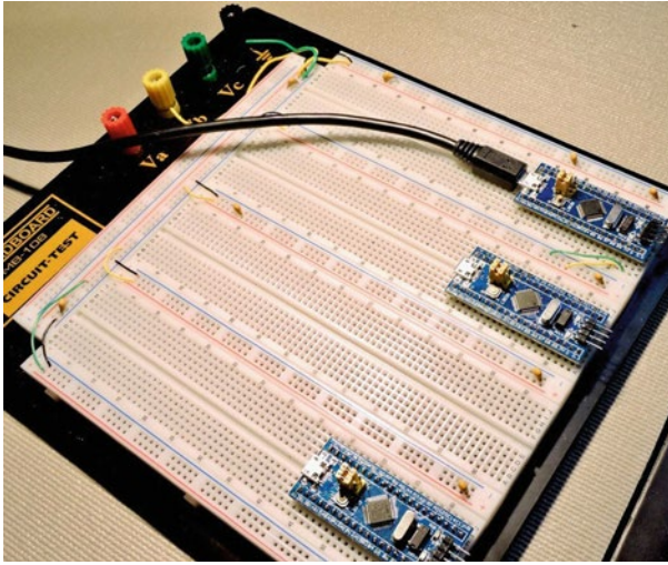
Figure 1-3. A breadboard with supply rails
