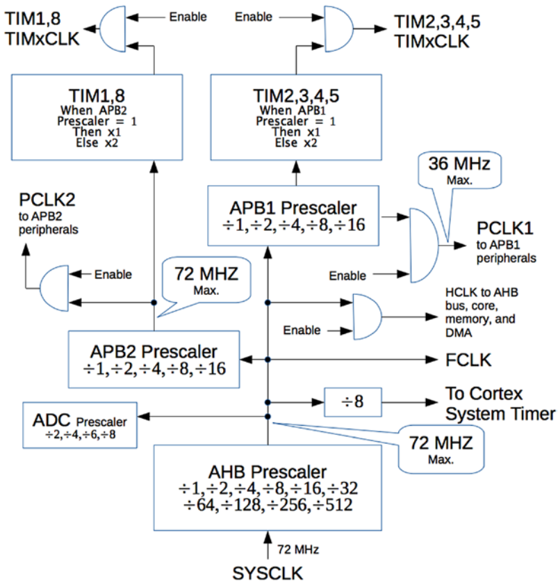
Figure 15-3. Clock tree starting from SYSCLK
