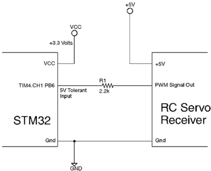
Figure 17-2. RC servo receiver hookup to STM32
