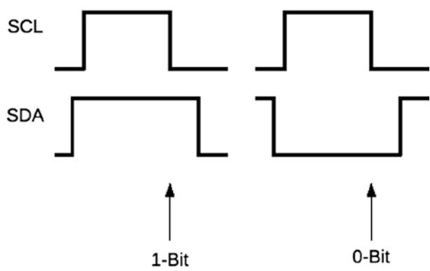
Figure 11-2. I2C data bit signals
