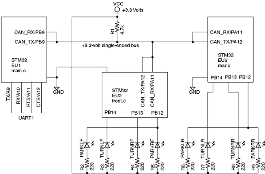
Figure 18-4. Demonstration CAN bus project hookup
