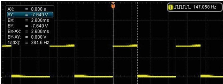
Figure 16-2. A PWM signal with a period of 147 Hz and a pulse width of 2.6 ms
