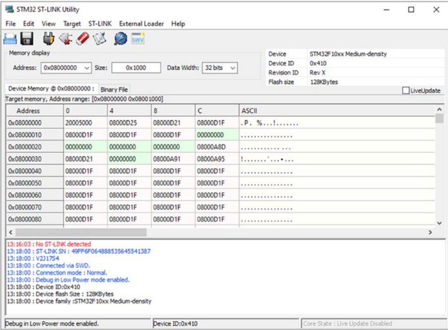
Figure 2-1. Example STM32 ST-LINK Utility display after connecting
