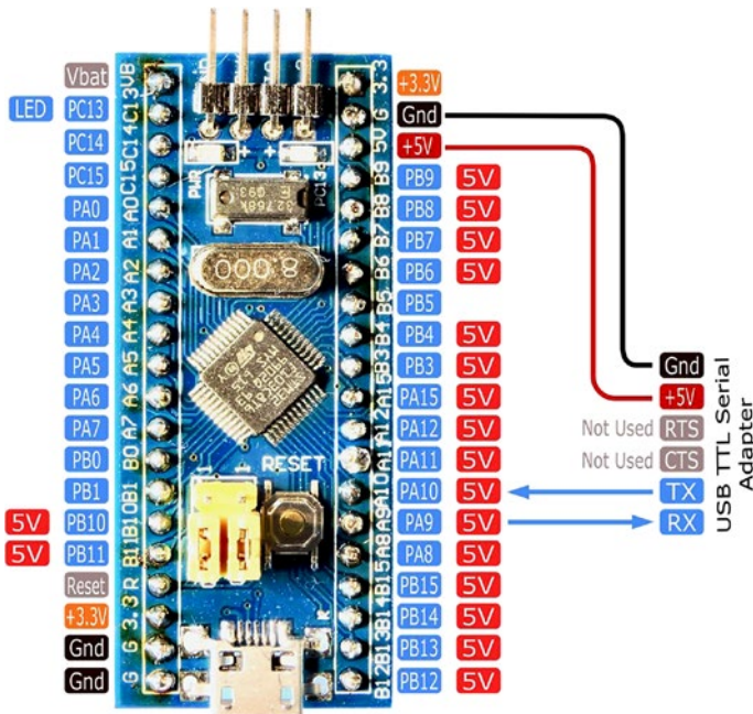
Figure 20-1. The UART hookup diagram
