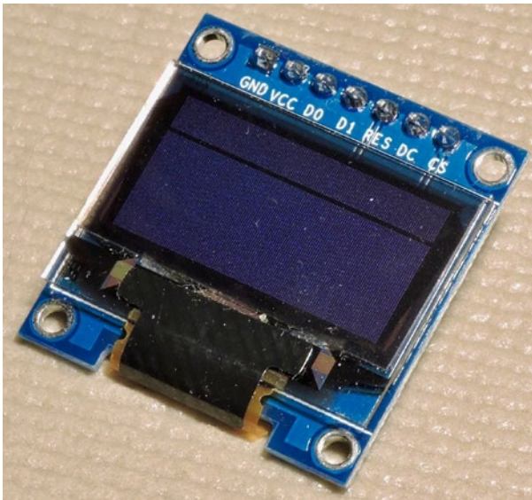
Figure 12-1. The OLED using an SSD1306 controller
