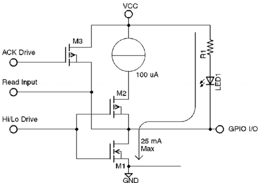
Figure 11-8. Driving higher-current loads with the PCF8574
