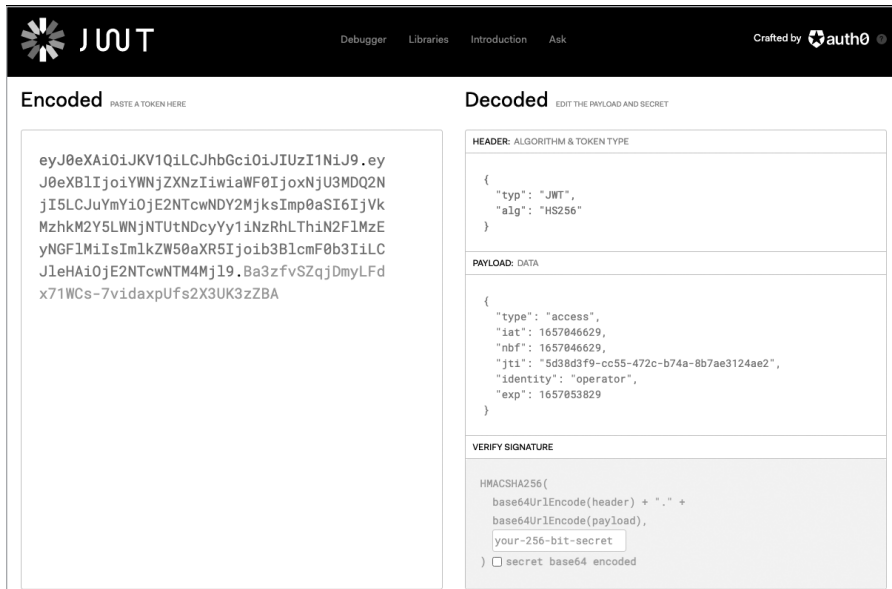
Figure 7-3: The DVGA operator's accessToken , decoded using https://jwt.io
