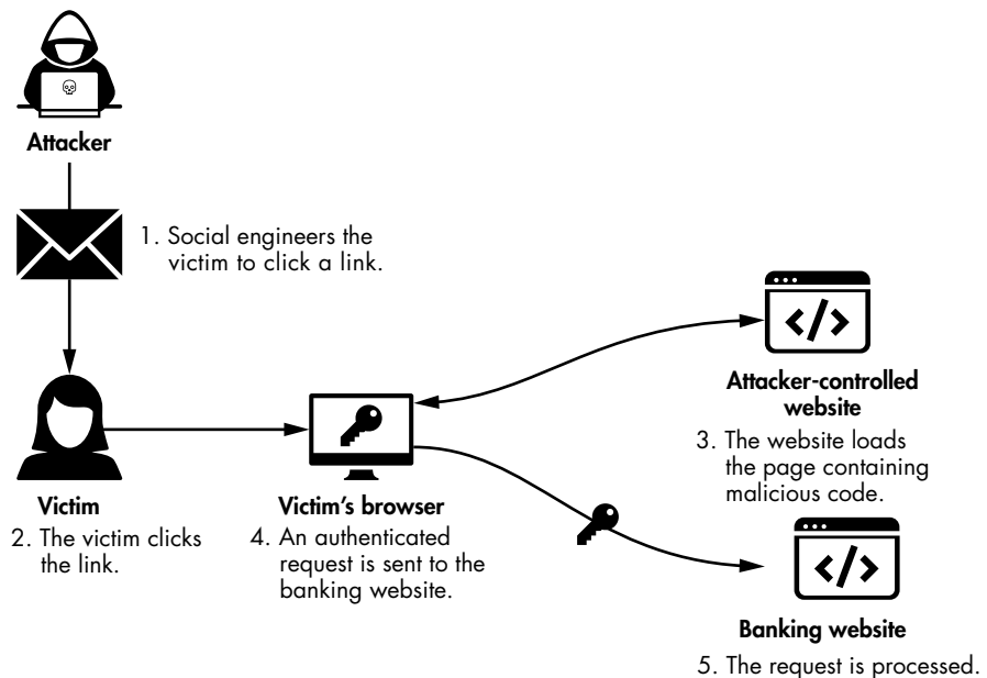
Figure 9-1: The flow of a CSRF attack
