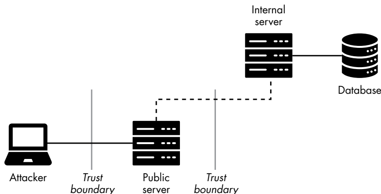
Figure 8-1: Network trust boundaries
