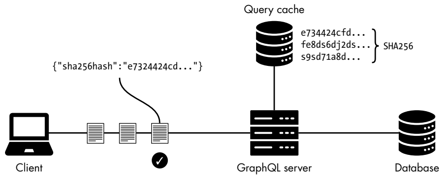
Figure 5-8: The APQ architecture
