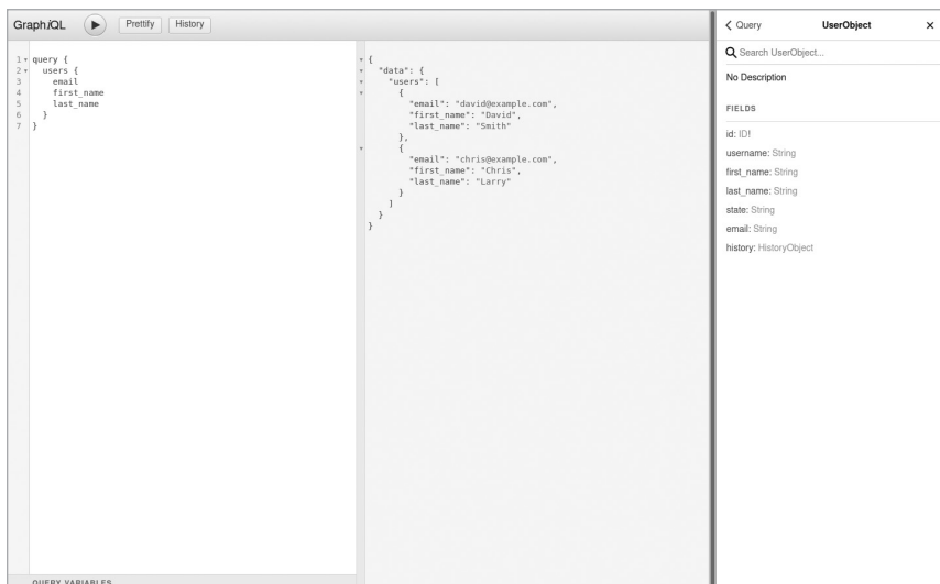
Figure 1-9: GraphQL Explorer autogenerated schema documentation
