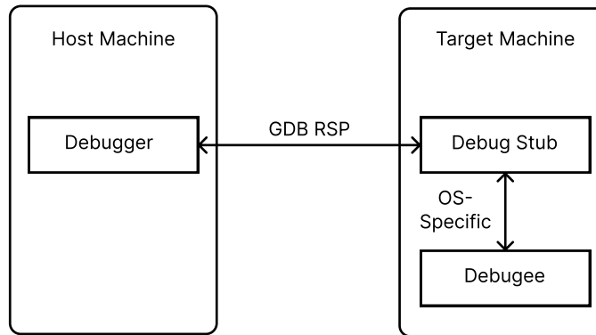
Figure 22-1: A remote debugging architecture
