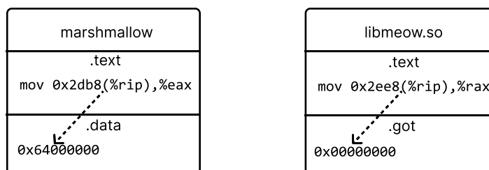
Figure 17-1: References between object files before relocation
