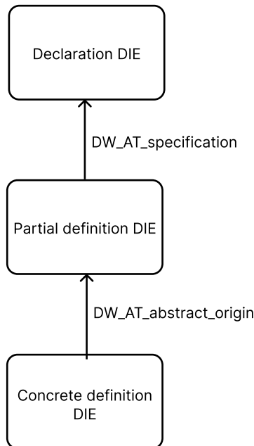
Figure 21-1: A chain of member function DIEs
