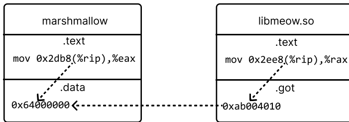
Figure 17-2: References between object files after relocation
