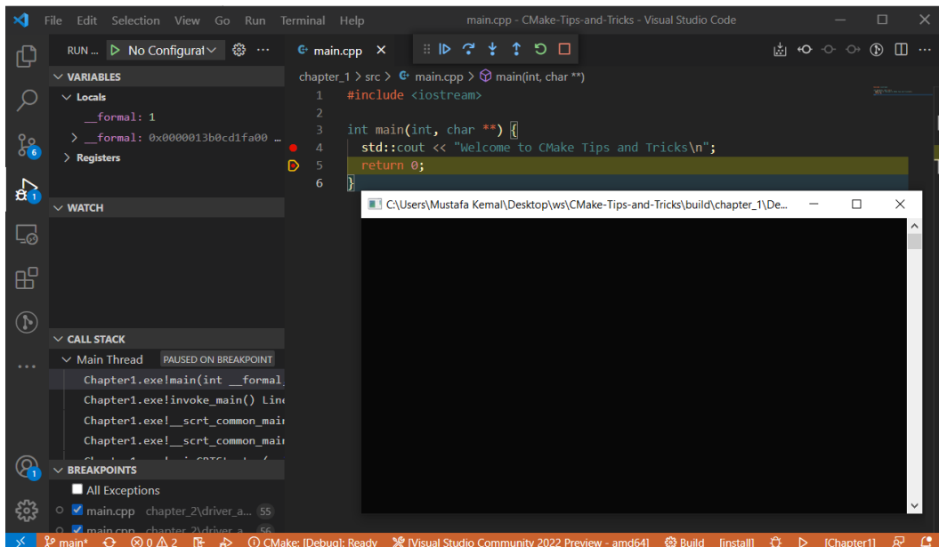
Figure 2.46 – Executable Chapter1 target being debugged
