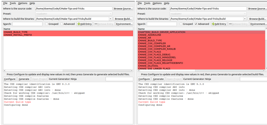
Figure 1.4 – Left – cmake-gui does not show variables marked as advanced. Right – Marking the "Advanced" checkbox displays all the variables marked as advanced
