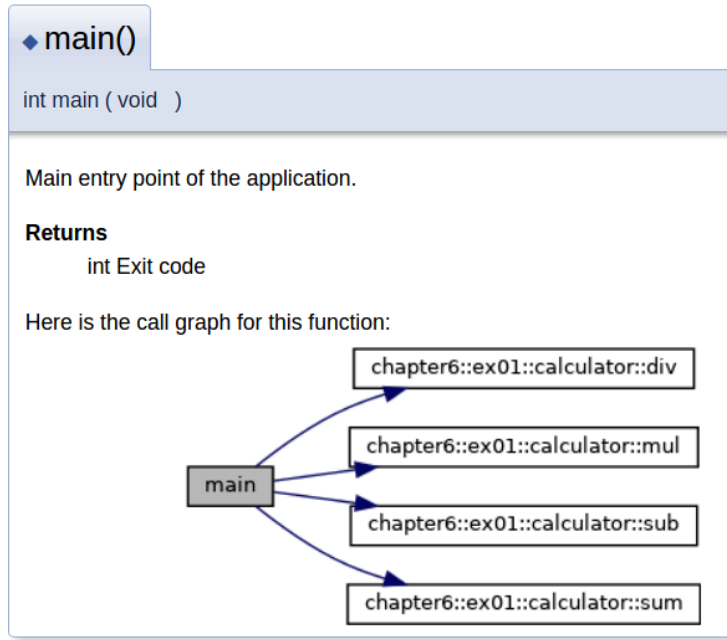
Figure 6.5 – main() function call graph
