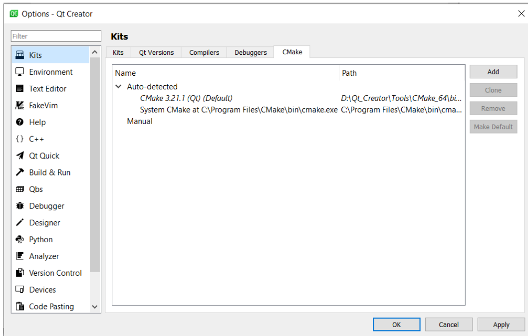
Figure 2.48 – Qt Creator CMake path settings
