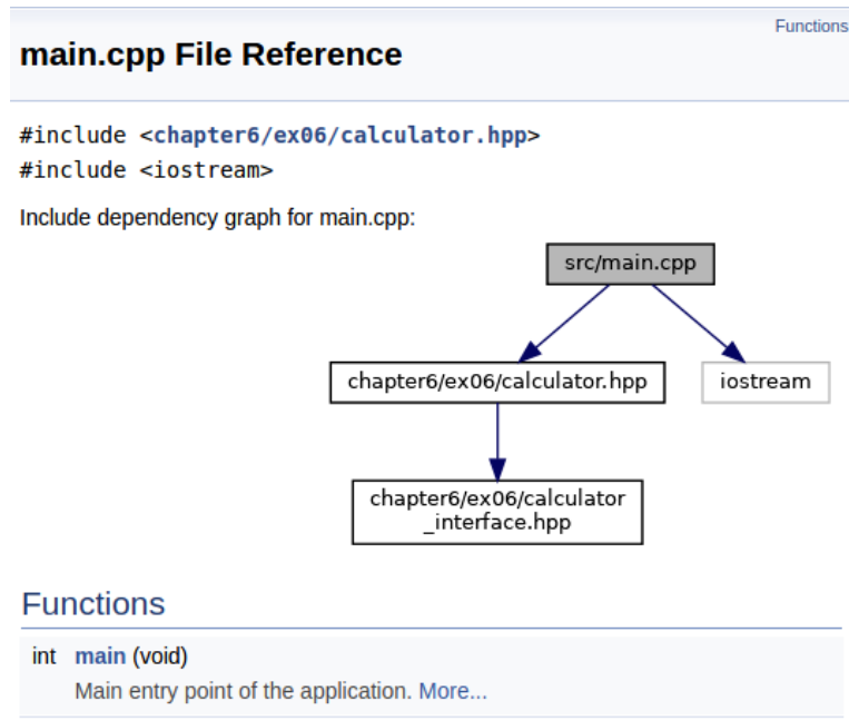
Figure 6.4 – main.cpp documentation page
