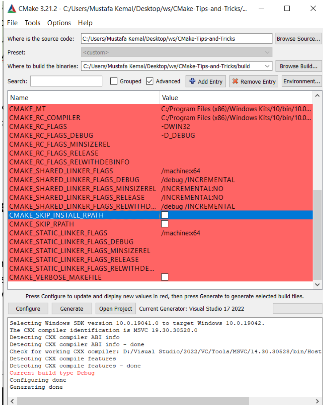
Figure 2.32 – cmake-gui in advanced mode
