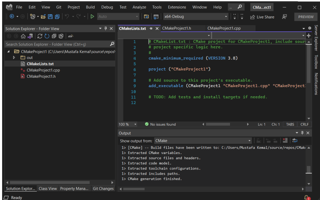
Figure 2.38 – First glance after creating a new CMake project with Visual Studio
