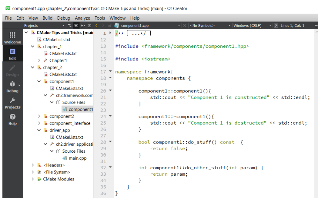
Figure 2.53 – A glance at the CMake Tips and Tricks example project in Qt Creator
