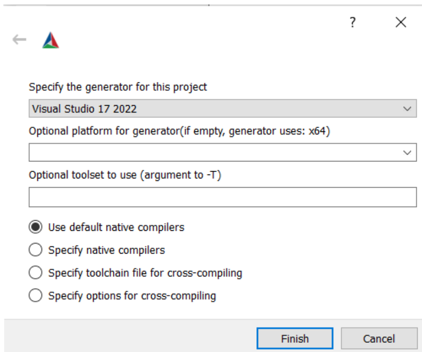
Figure 2.30 – CMake GUI generator selection screen
