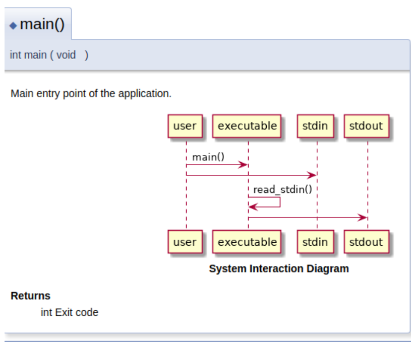
Figure 6.6 – Embedded PlantUML diagram in the main() function documentation
