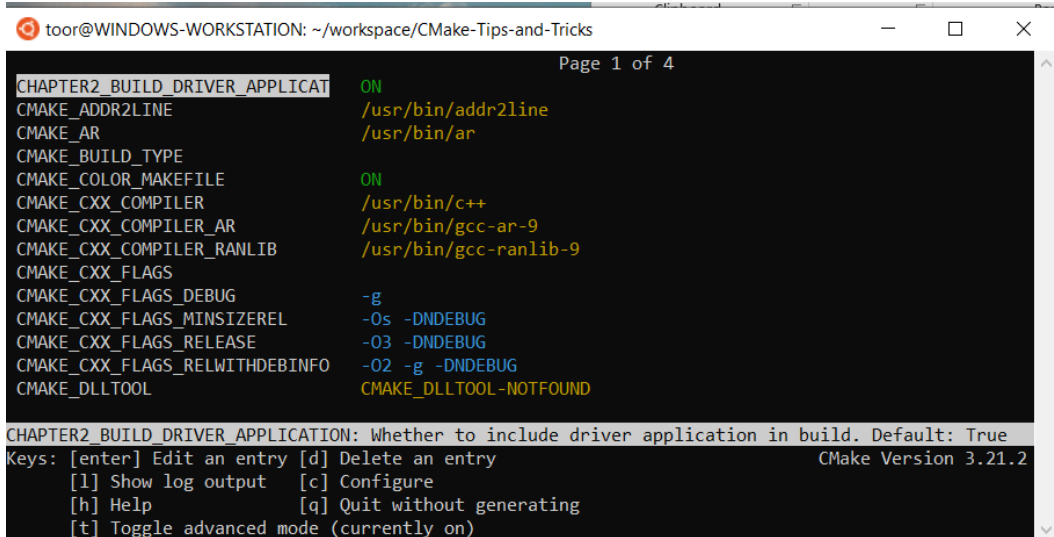
Figure 2.28 – cmake in advanced mode
