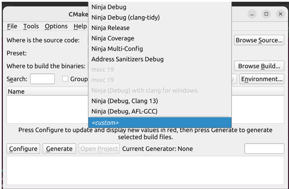
Figure 9.1 – Listing available presets in the CMake GUI
