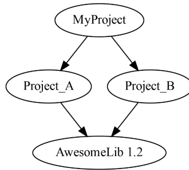
Figure 5.2 – The corrected dependency graph after MyProject declares the version of AwesomeLib
