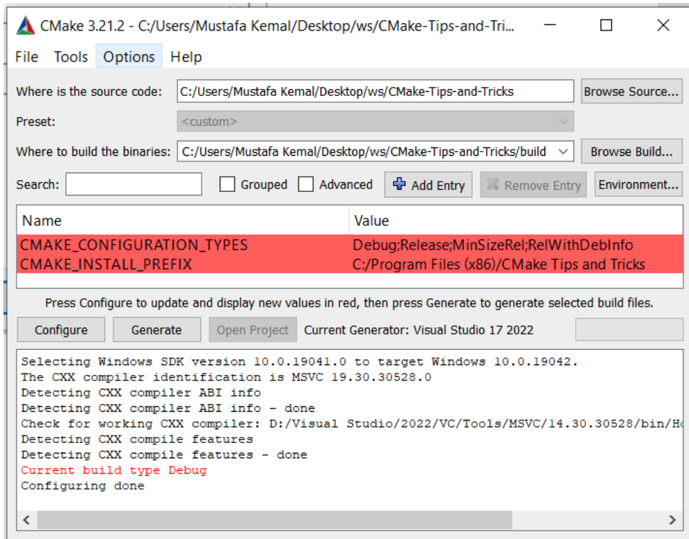
Figure 2.31 – CMake GUI after configuration
