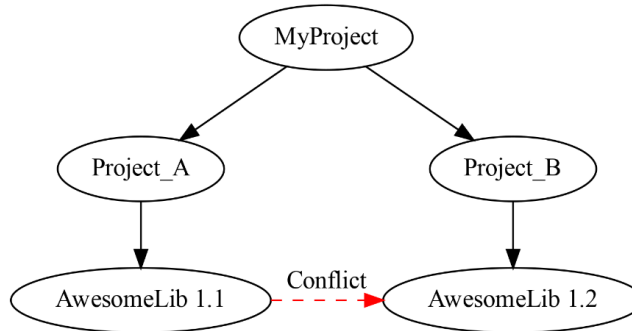
Figure 5.1 – Both Project_A and Project_B depend on different versions of AwesomeLib
