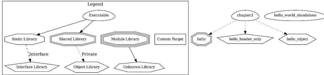
Figure 6.7 – The project structure of chapter3 visualized with the DOT language
