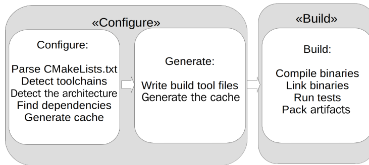
Figure 1.3 – CMake's two-stage build process
