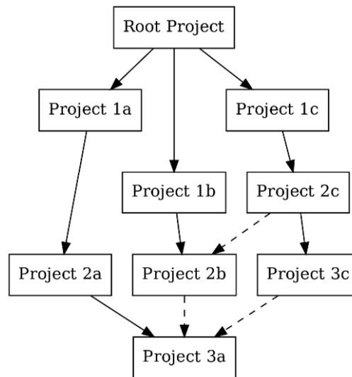
Figure 15.1 – An example project hierarchy showing the various dependencies
