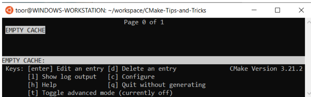
Figure 2.23 – ccmake main screen
