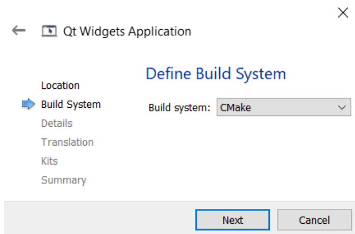
Figure 2.51 – Qt Creator new project wizard build system selection
