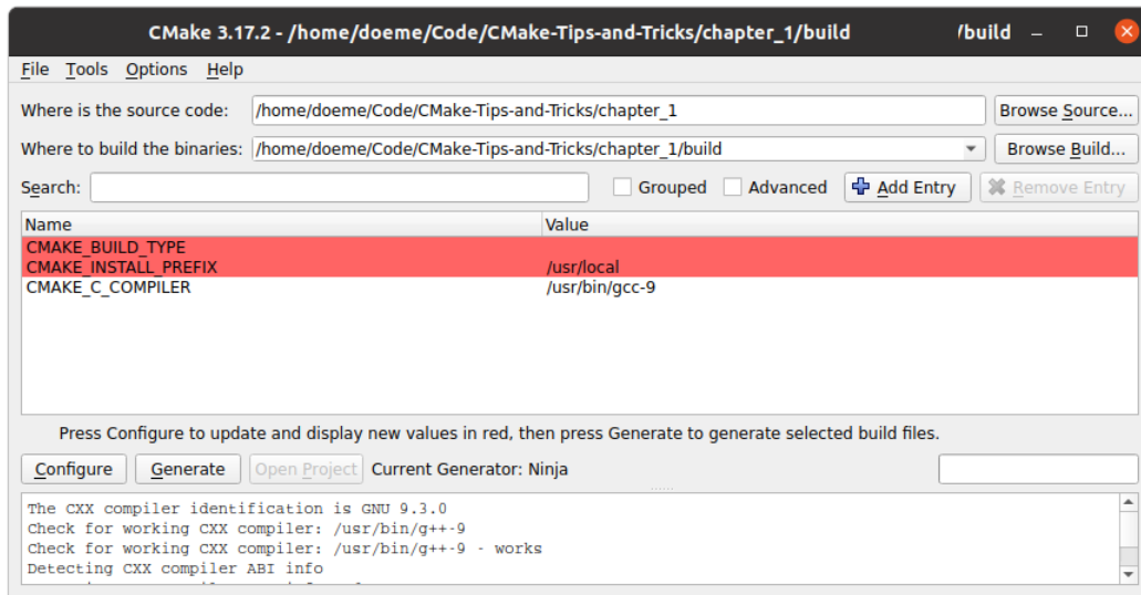
Figure 1.1 – cmake-gui after configuring a project
