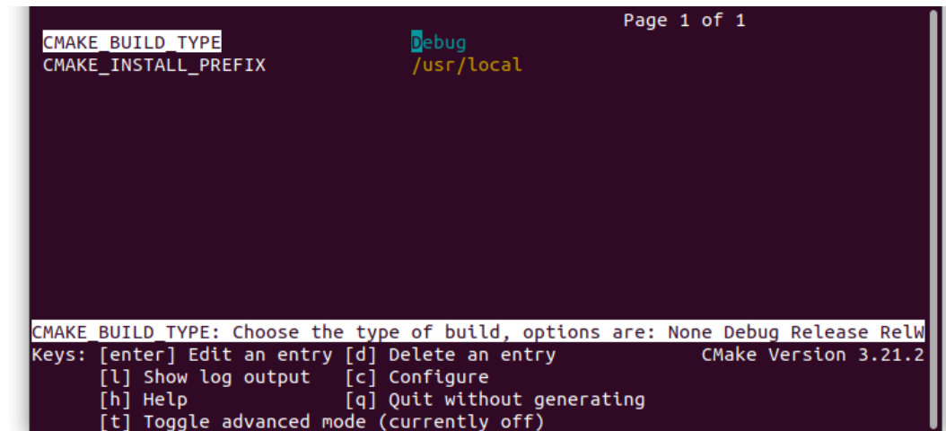
Figure 1.2 – Configuring a project using ccmake
