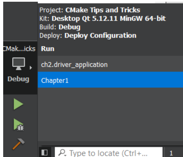
Figure 2.56 – Kit selector displaying CMake targets
