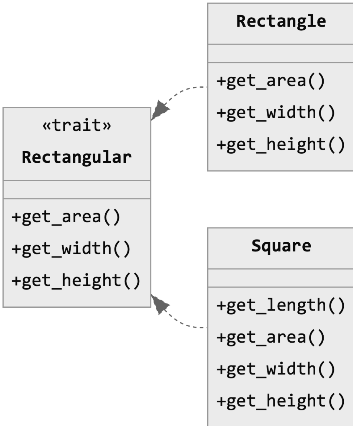
Figure 8.2 UML for Rust geometric shapes
