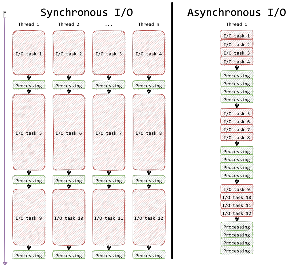
Figure 11.3 Comparing Synchronous to Asynchronous I/O
