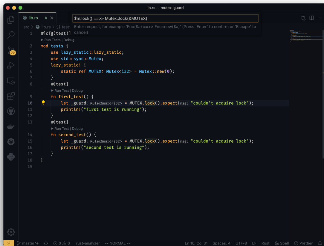
Figure 6.1 Structural substitution with rust-analyzer, before applying
