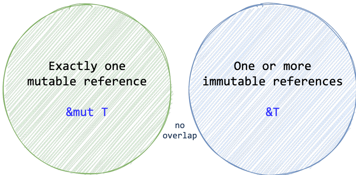
Figure 1.3 Rust borrow checker rules Venn diagram
