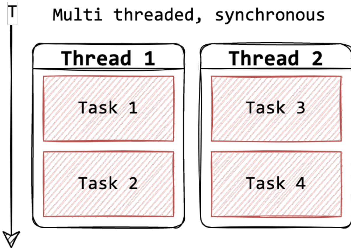
Figure 11.2 Synchronous tasks executing in parallel across 2 threads
