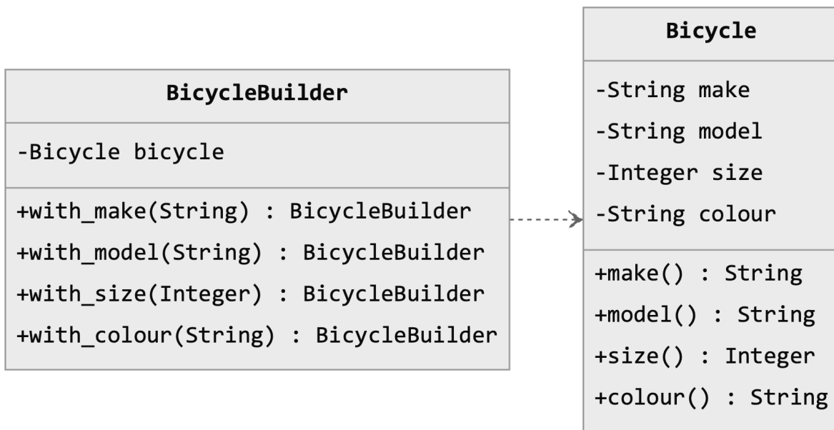
Figure 9.2 UML diagram for fluent builder pattern
