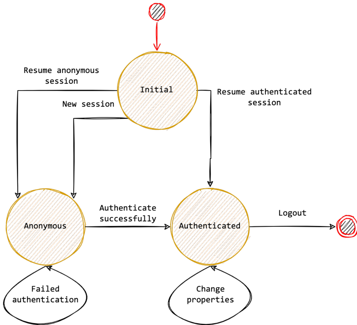
Figure 10.1 Modeling a user session with a state machine
