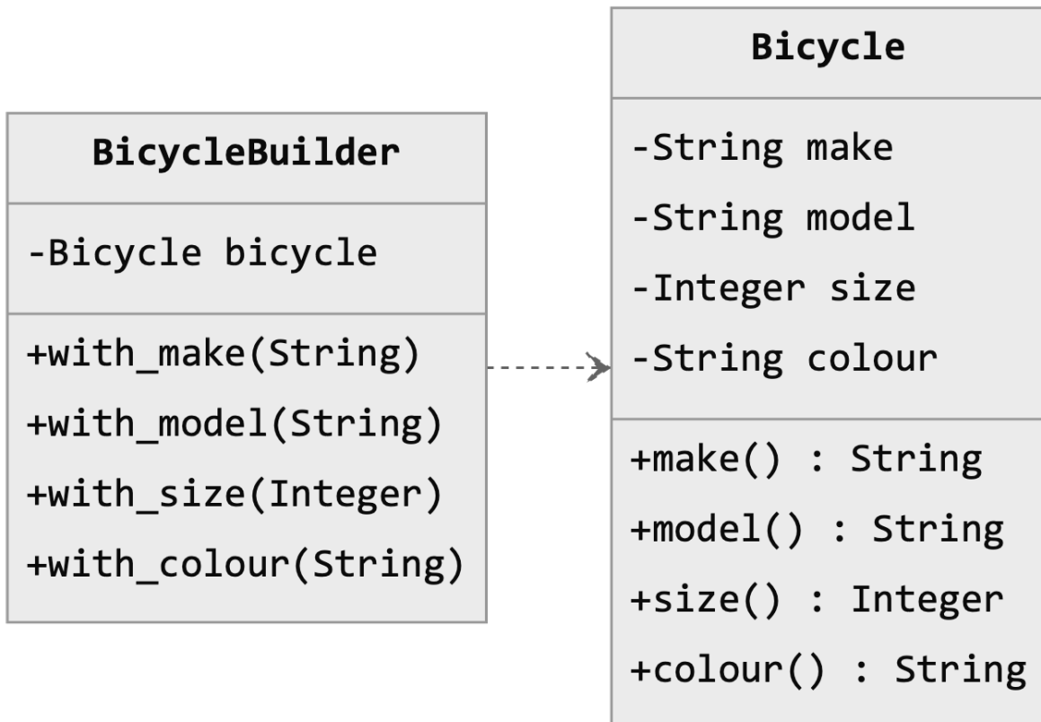
Figure 9.1 UML diagram for builder pattern
