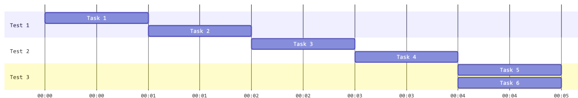
Figure 11.4 Diagram showing sequence of events with blocking sleep
