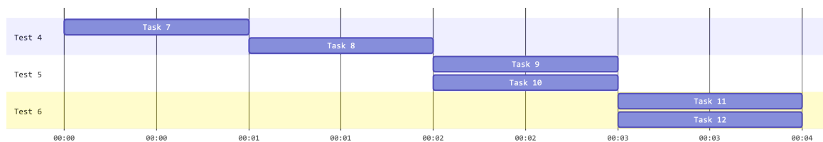
Figure 11.5 Diagram showing sequence of events with non-blocking sleep
