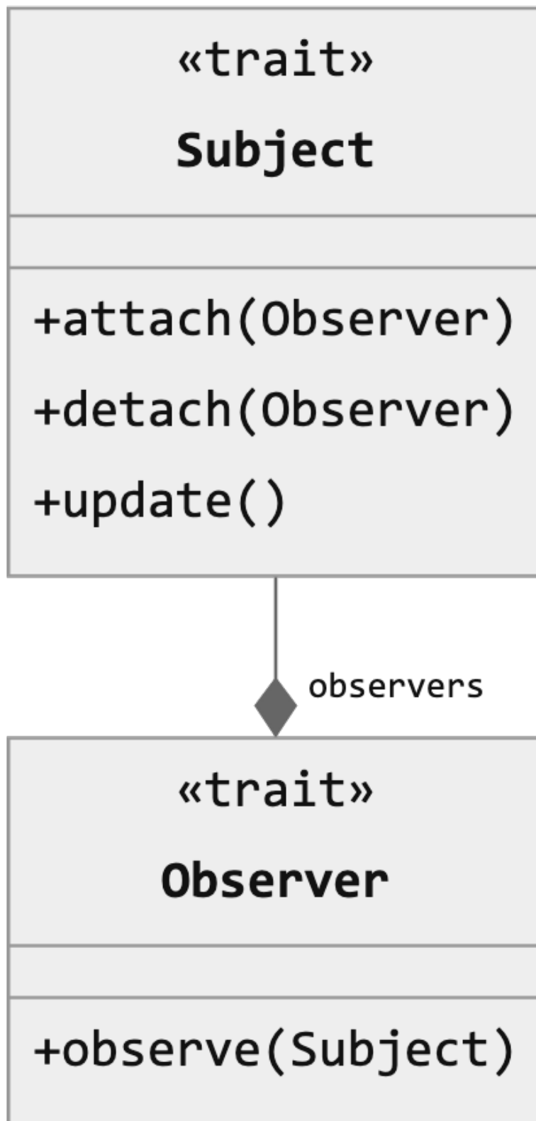
Figure 9.3 UML diagram for observer pattern
