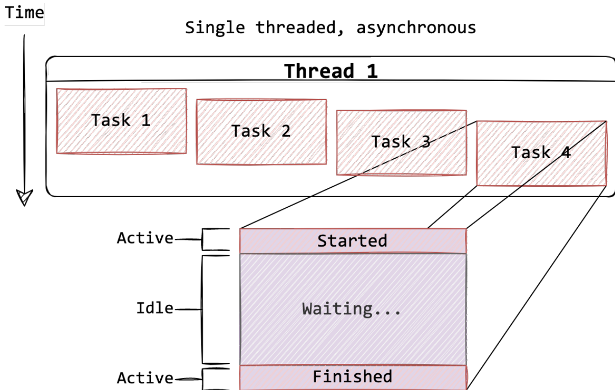
Figure 11.1 Tasks executing concurrently within the same thread
