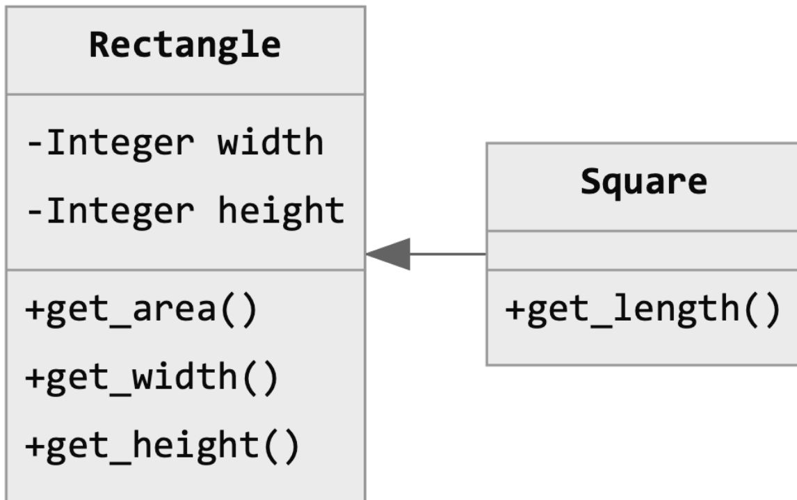
Figure 8.1 UML diagram for C++ geometric shapes
