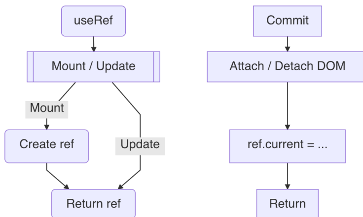
Figure 8.3 – useRef workflow
