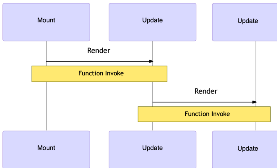
Figure 2.3 – React render for a function component
