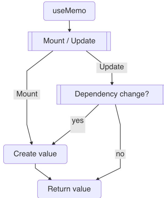
Figure 6.2 – useMemo workflow
