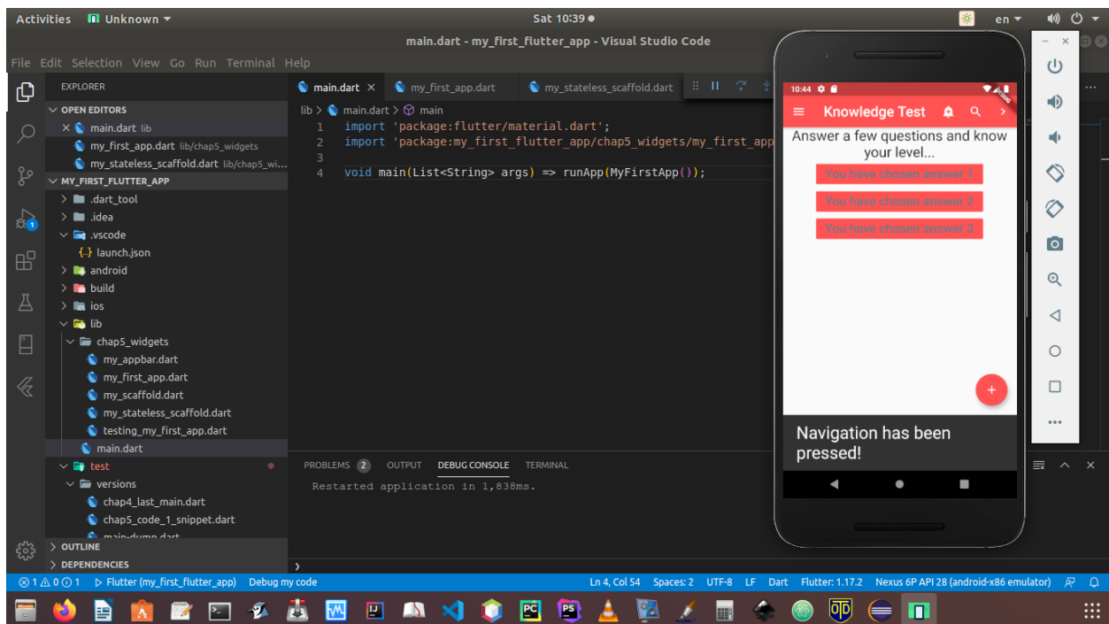
Figure 5.3 – A complete new look of 'appbar' widget, where widget state has been managed
