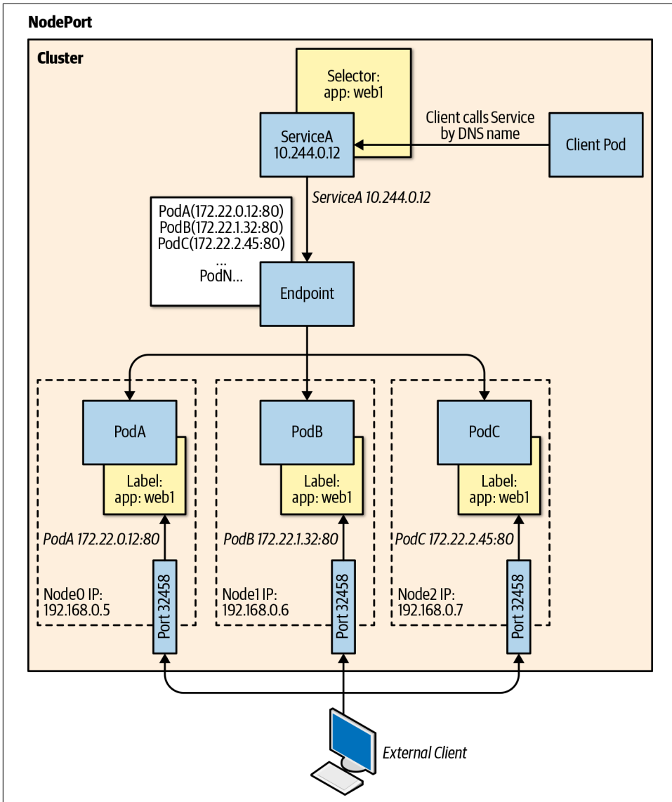
Figure 9-5. NodePort-Pod, Service and Host network visualization
