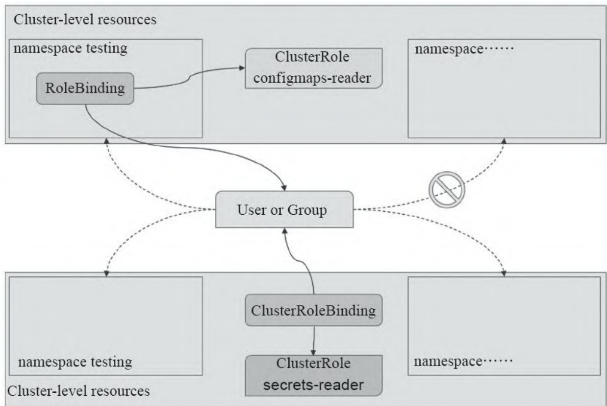
图10-12 RoleBinding与ClusterRoleBinding
