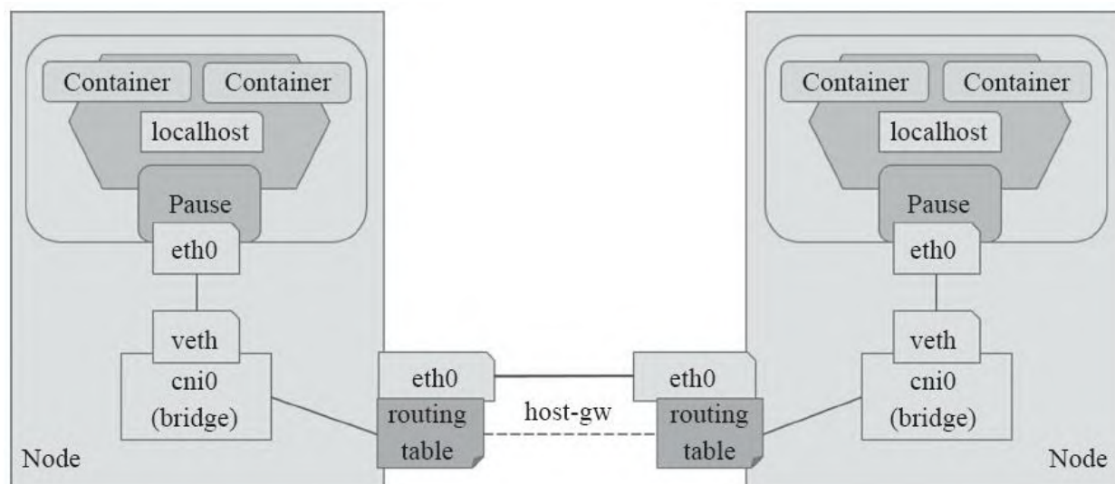
图11-10 host-gw后端
