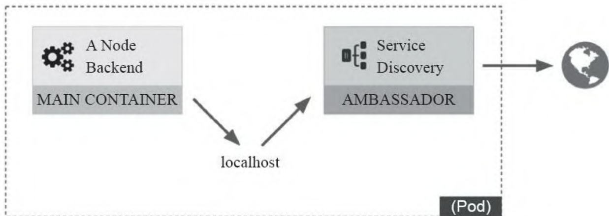
图4-3 Ambassador pattern
