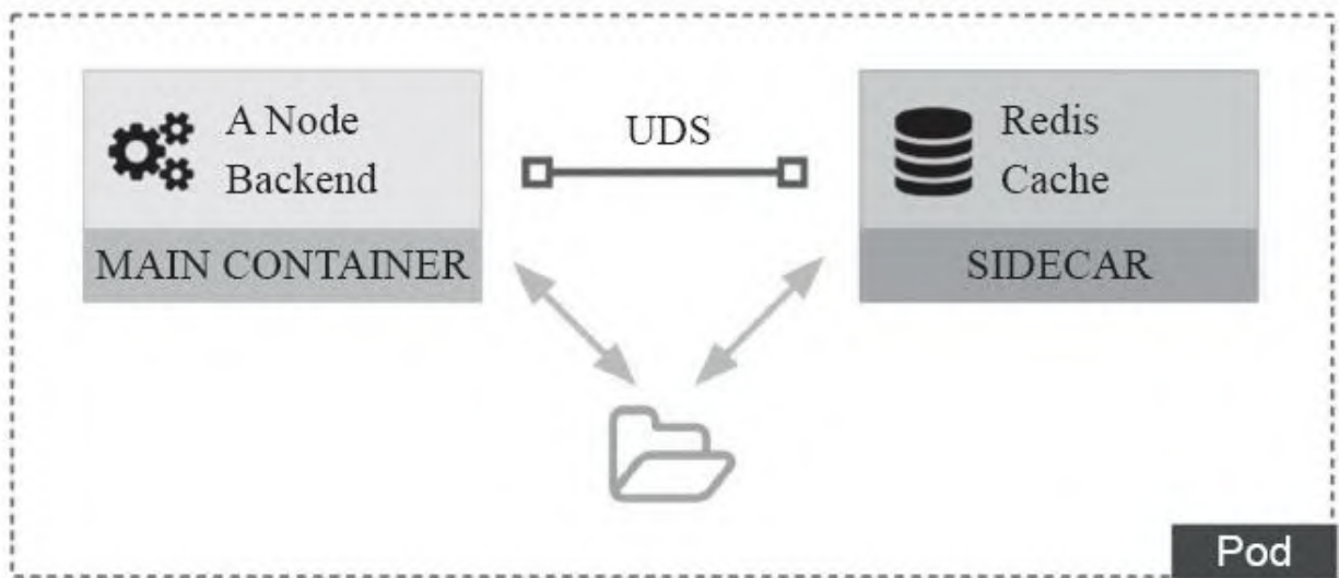
图4-2 Sidecar pattern
