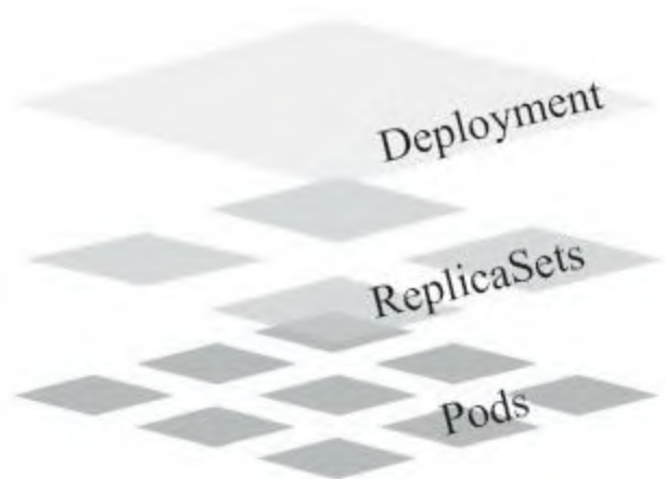
图5-7 Deployment、ReplicaSets和Pods
