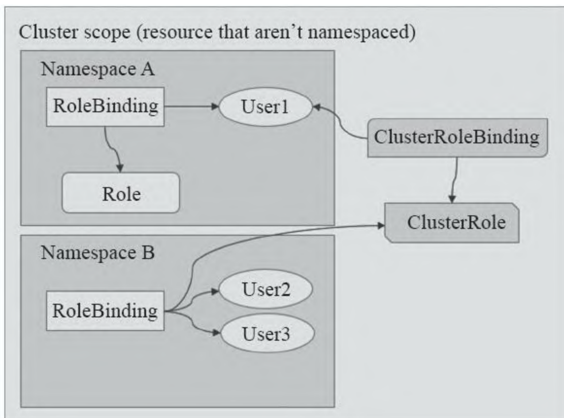
图10-11 Role、RoleBinding、ClusterRole和ClusterRoleBinding
