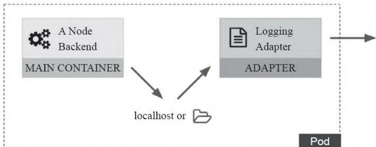
图4-4 Adapter pattern
