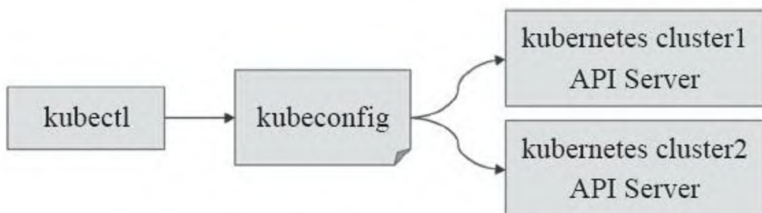
图10-5 kubectl和kubecofnig
