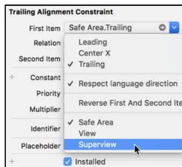
Edit Auto Layout constraint
