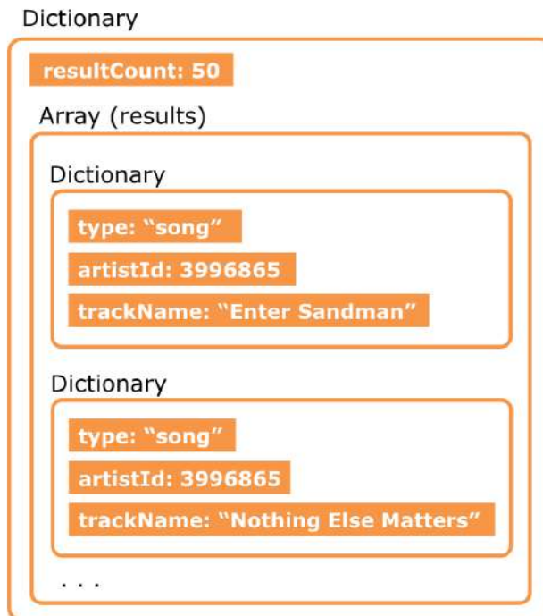
The structure of the JSON data
