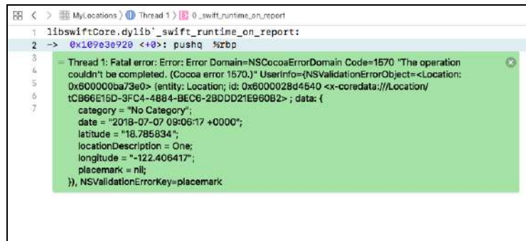
The app crashes after a Core Data error
