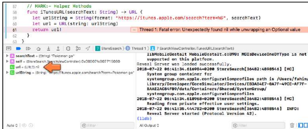
The crash after searching for pokemon-go
