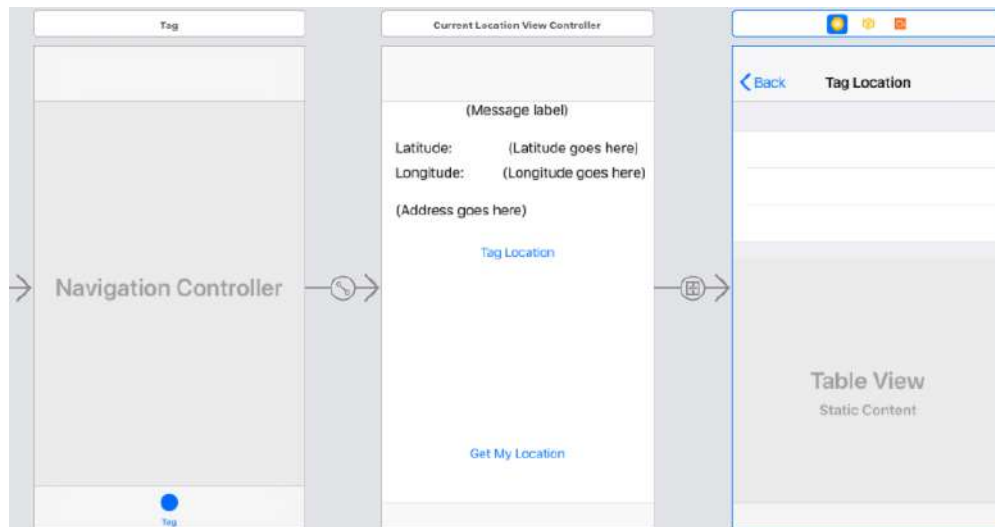
The Tag Location screen in the storyboard
