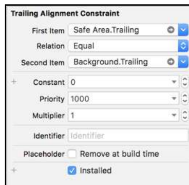
Auto Layout constraint editor
