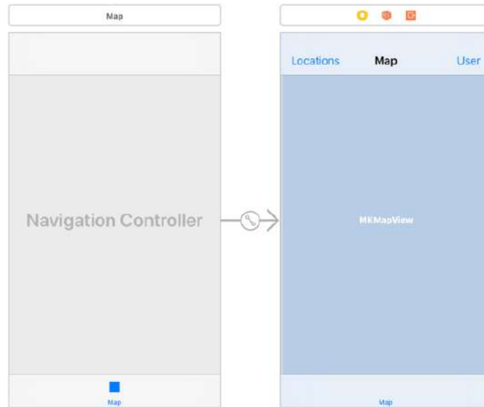
The design of the Map screen
