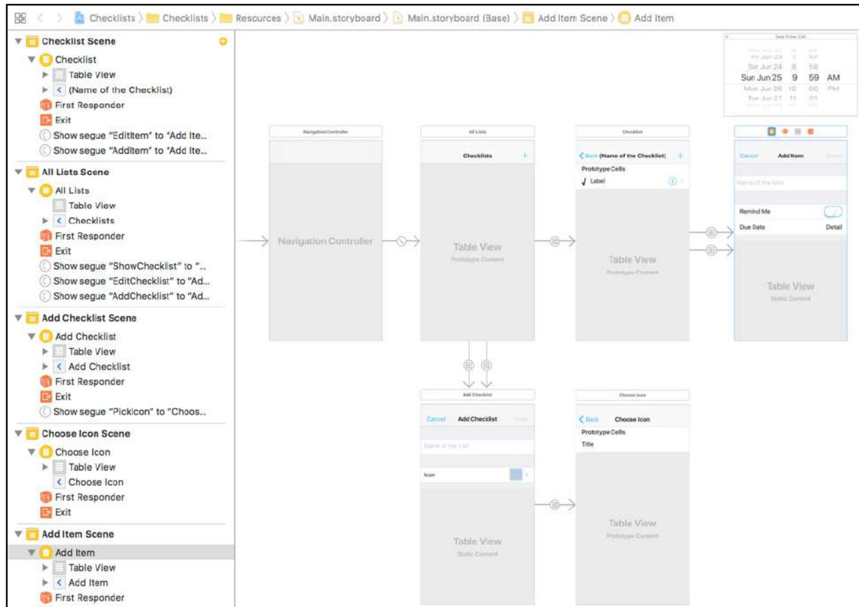
The final storyboard
