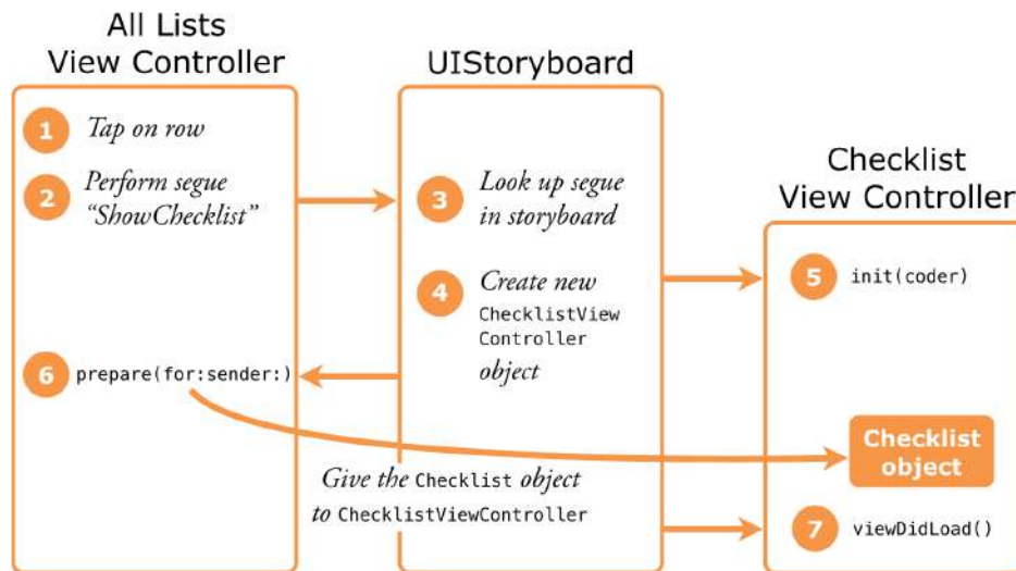
The steps involved in performing a segue
