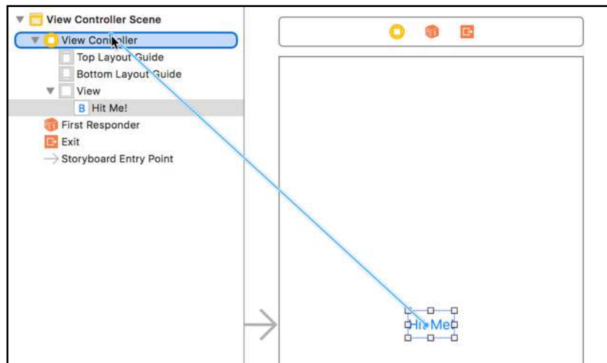
Ctrl-drag from the button to View Controller
