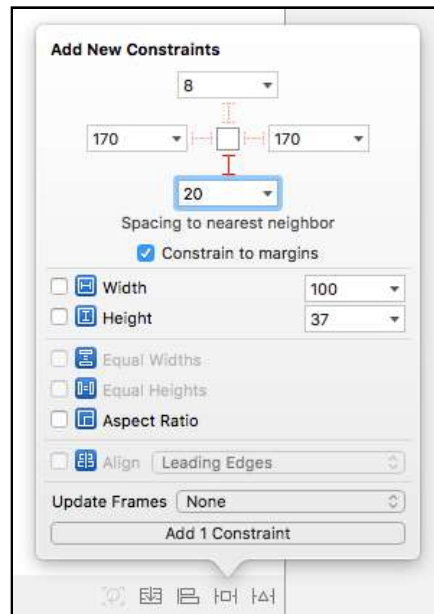
The red I-beams decide the sides that are pinned down
