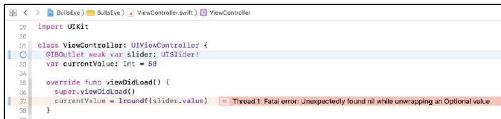
App crash when outlet is not connected
