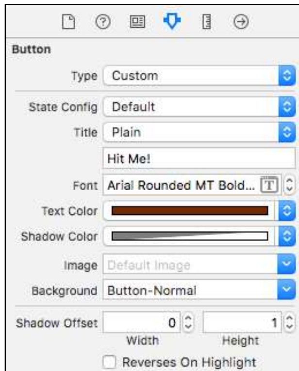
The attributes for the Hit Me! button in the default state
