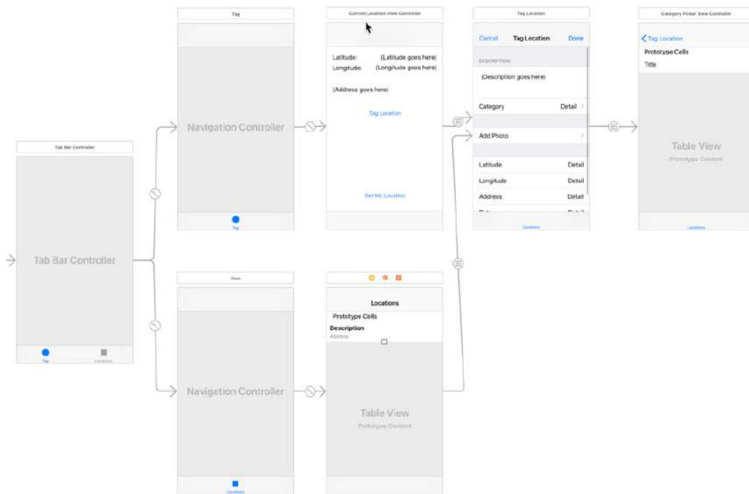
The Location Details screen is now also connected to the Locations screen
