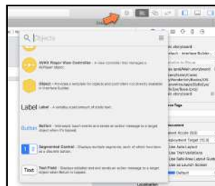
The Object Library
