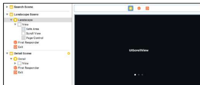
The final design of the Landscape scene
