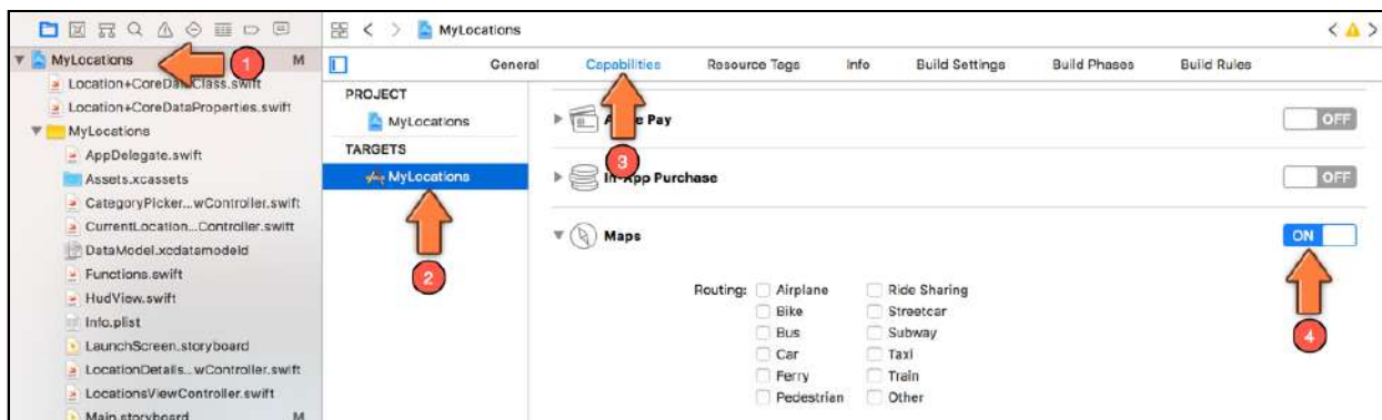
Enabling the app to use maps
