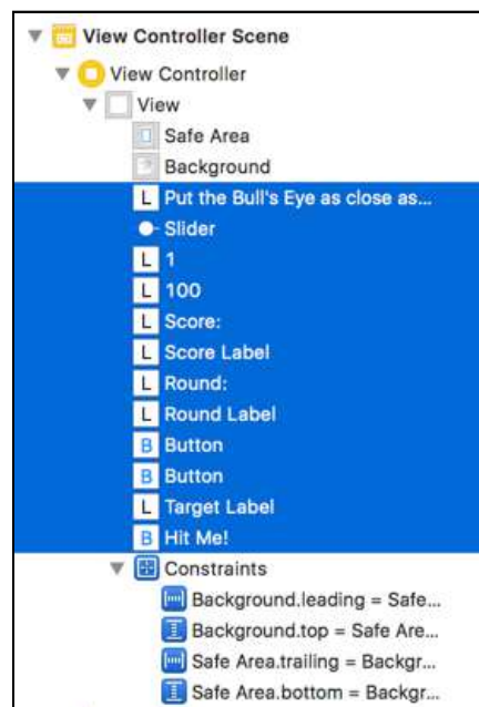
Selecting the views from the Document Outline
