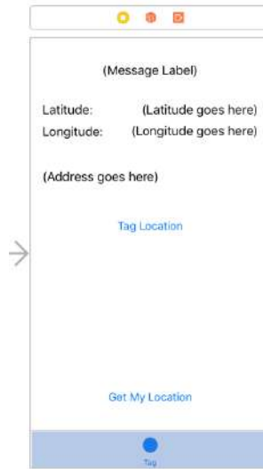
The design of the Current Location screen
