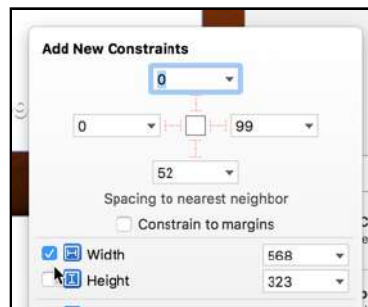
Pinning the width and height of the container view
