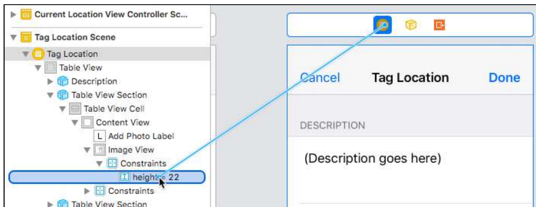
Connect the outlet for the constraint
