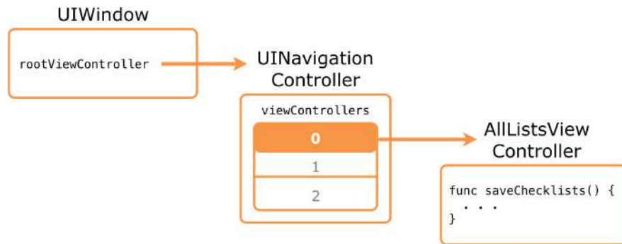
From the root view controller to the AllListsViewController
