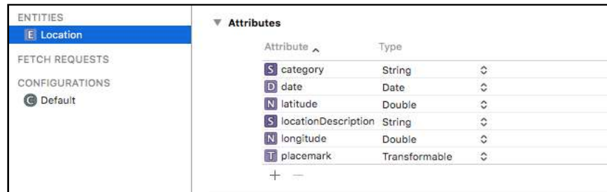
All the attributes of the Location entity
