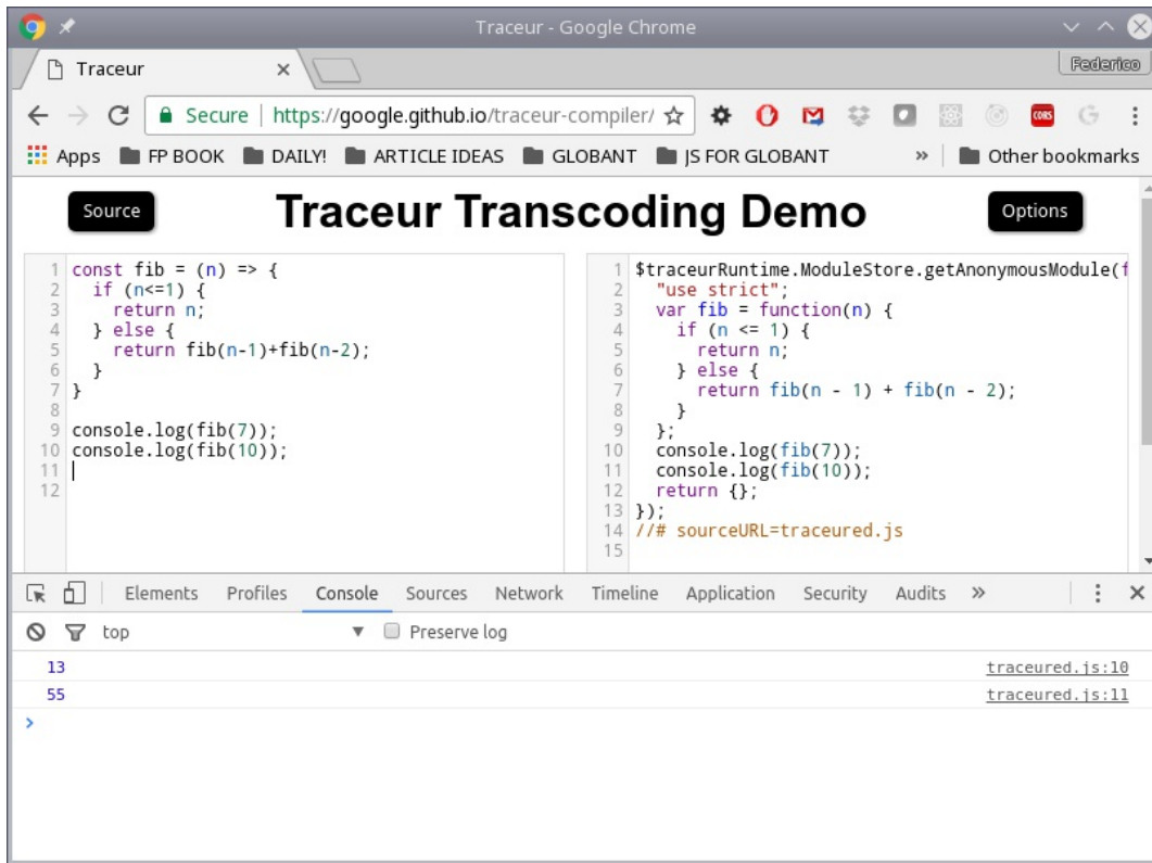
Figure 1.3 - The Traceur transpiler is an equally valid alternative for ES8-to-JS5 translation
