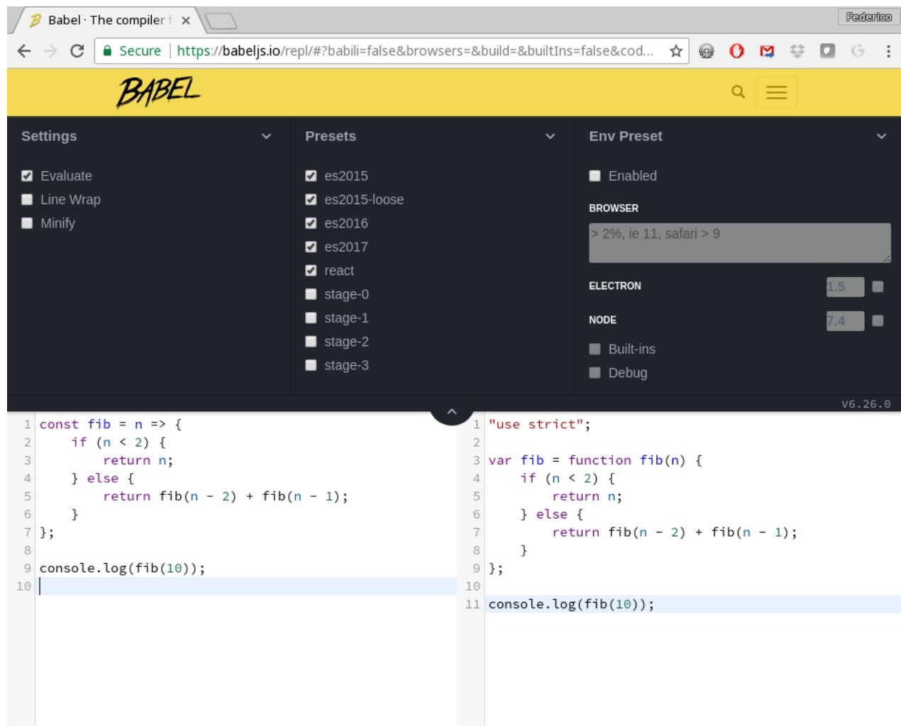
Figure 1.2 - The Babel transpiler converts ES8 code into compatible JS5 code
