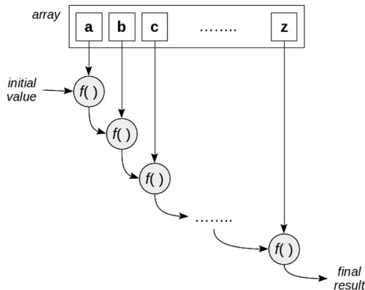
Figure 5.1: The reduce operation traverses the array, applying a function to each element and to the accumulated value
