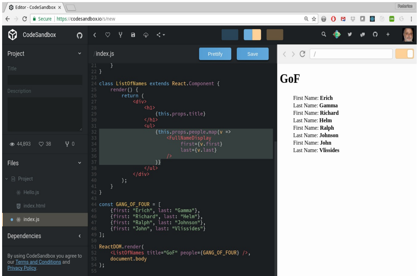
Figure 11.1: The original version of our components shows a (not much to speak about) list of names
