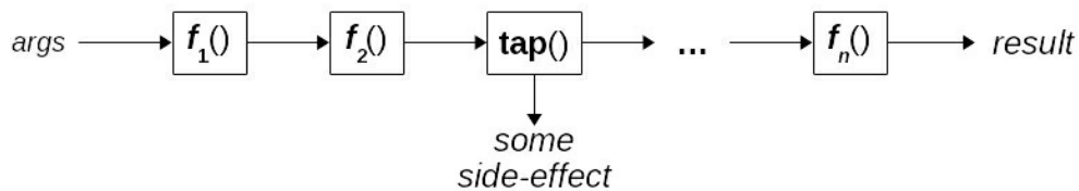
Figure 8.2. Tapping allows you to apply some function to inspect data as it flows through the pipeline.
