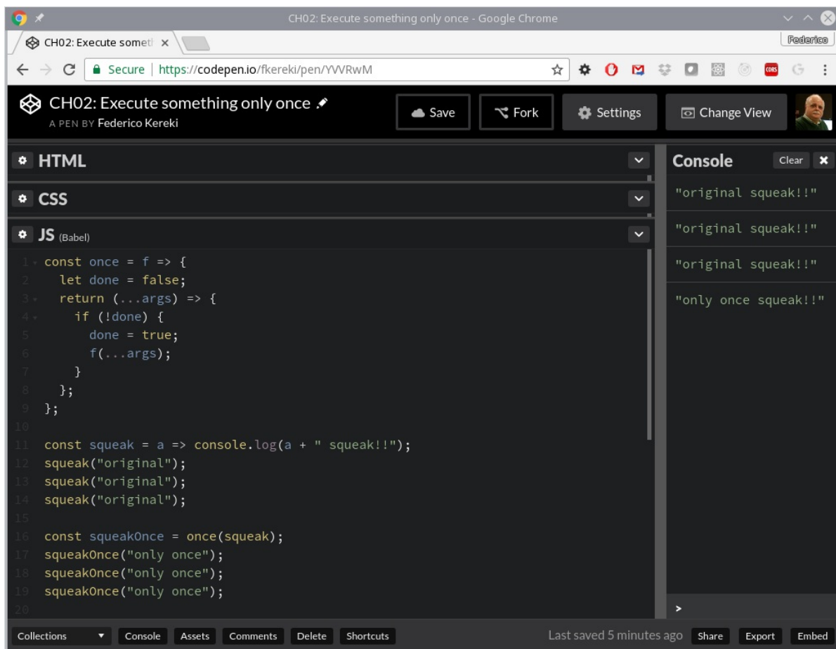
Figure 2.2 - Testing our once() higher-order function
