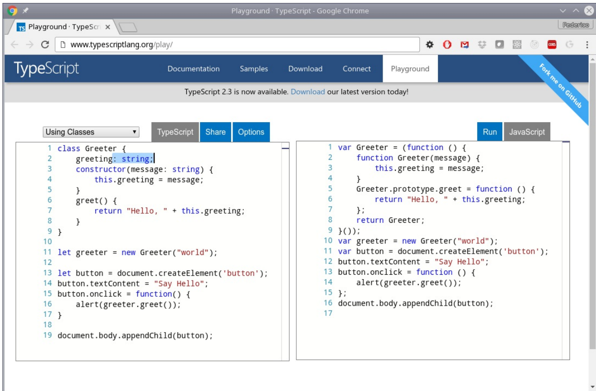
Figure 1.4 - TypeScript adds type checking features, for safer JS programming
