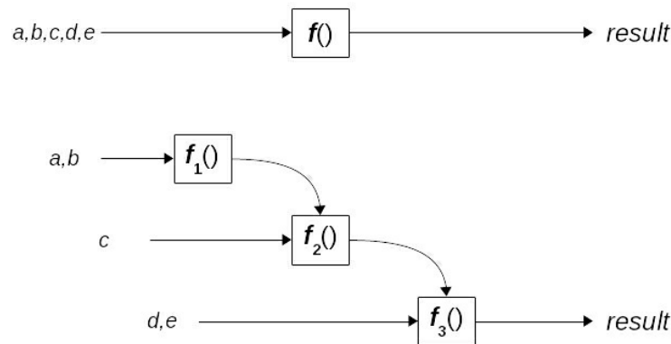
Figure 7.3. "Partial currying" is a mixture of currying and partial application. You may provide arguments from the left, in any quantity, until all have been provided, and then the result is calculated.
