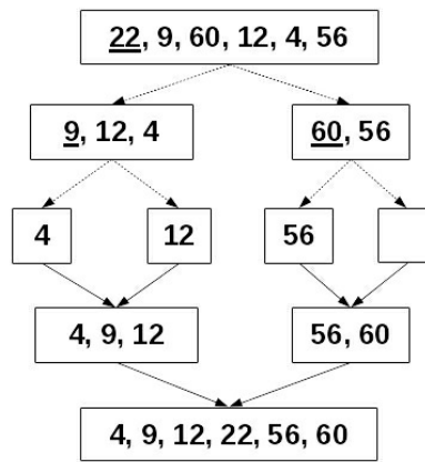
Figure 9.2. Quicksort sorts an array recursively, applying the divide and conquer strategy, to reduce the original problem to smaller ones.
