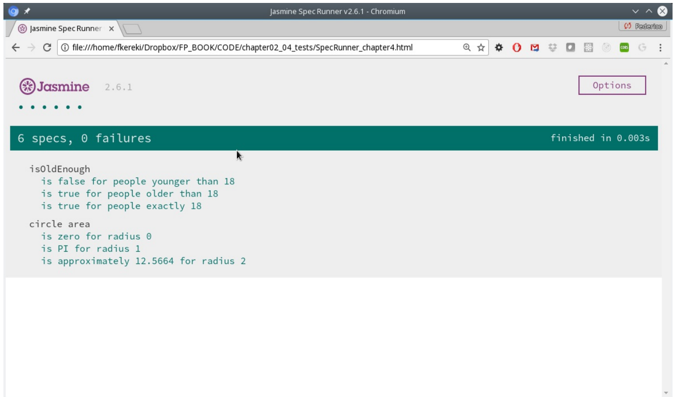
Figure 4.3: A successful test run for a pair of simple pure functions
