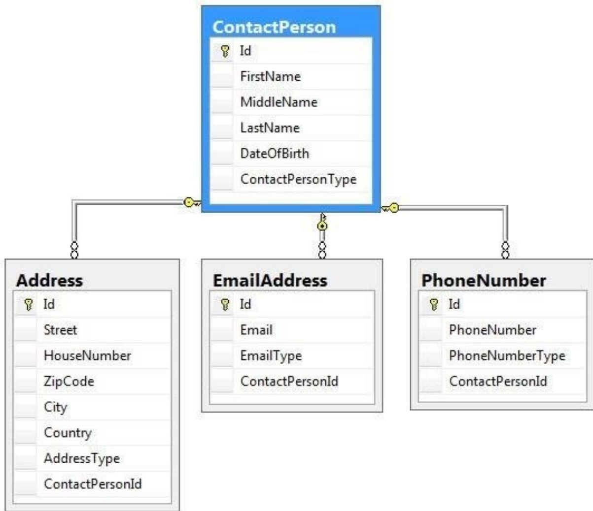
Relational Database Model
