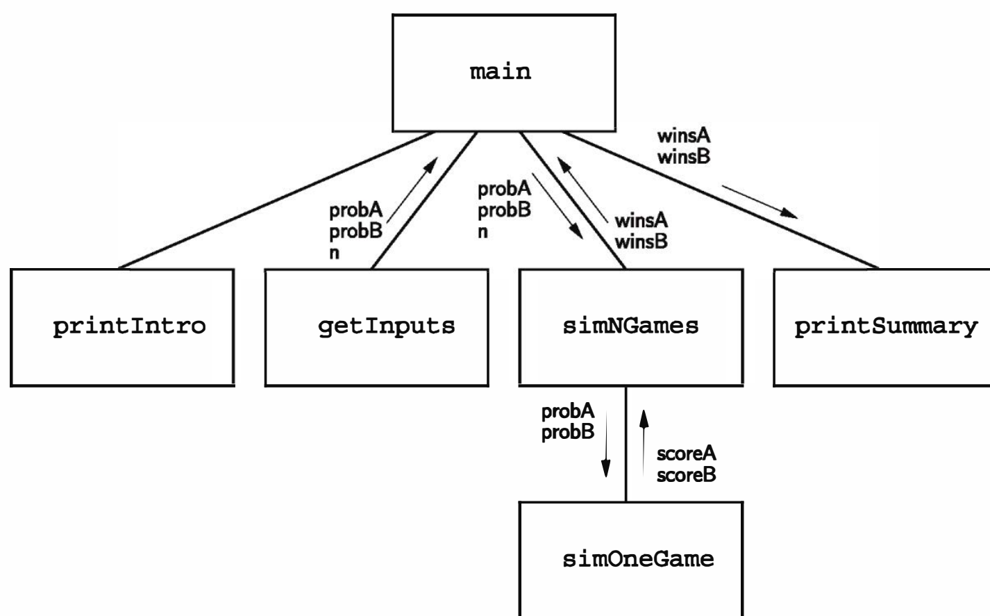
Figure 9.2: Second-level structure chart for racquetball simulation
