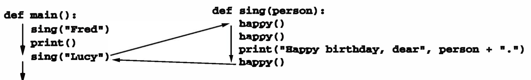
Figure 6.5: Completion of second call to sing
