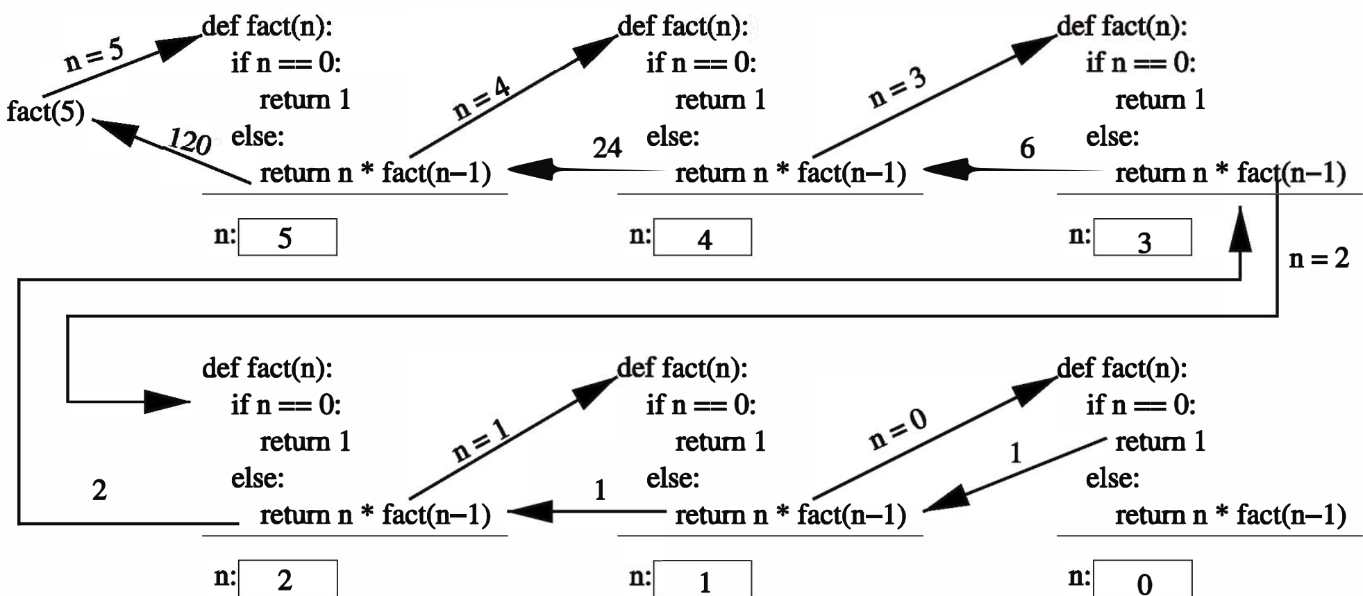
Figure 13.1: Recursive computation of 5!
