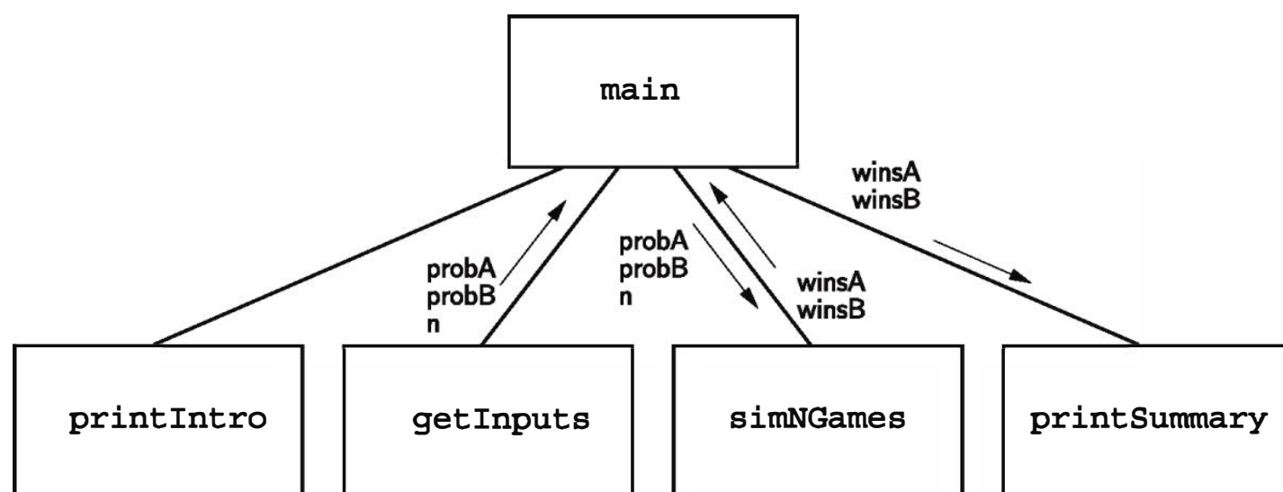
Figure 9.1: First-level structure chart for racquetball simulation
