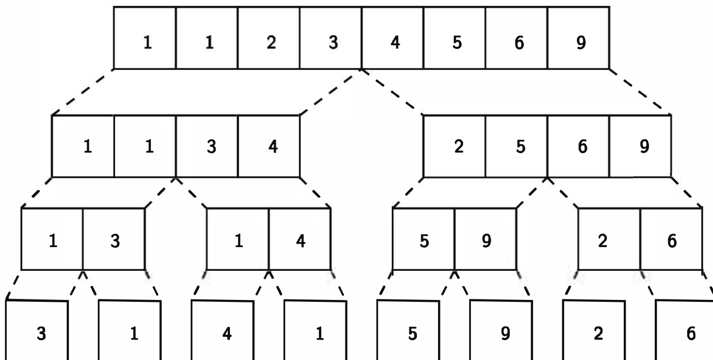
Figure 13.3: Merges required to sort [3, 1, 4, 1, 5, 9, 2, 6]
