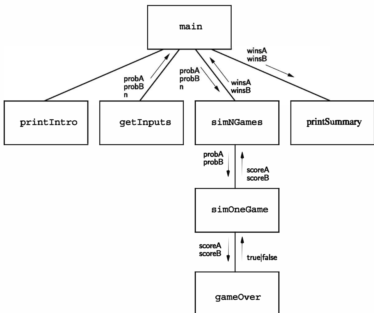
Figure 9.3: Third-level structure chart for racquetball simulation
