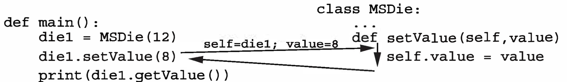
Figure 10.2: Flow of control in call: die1.setValue(8)
