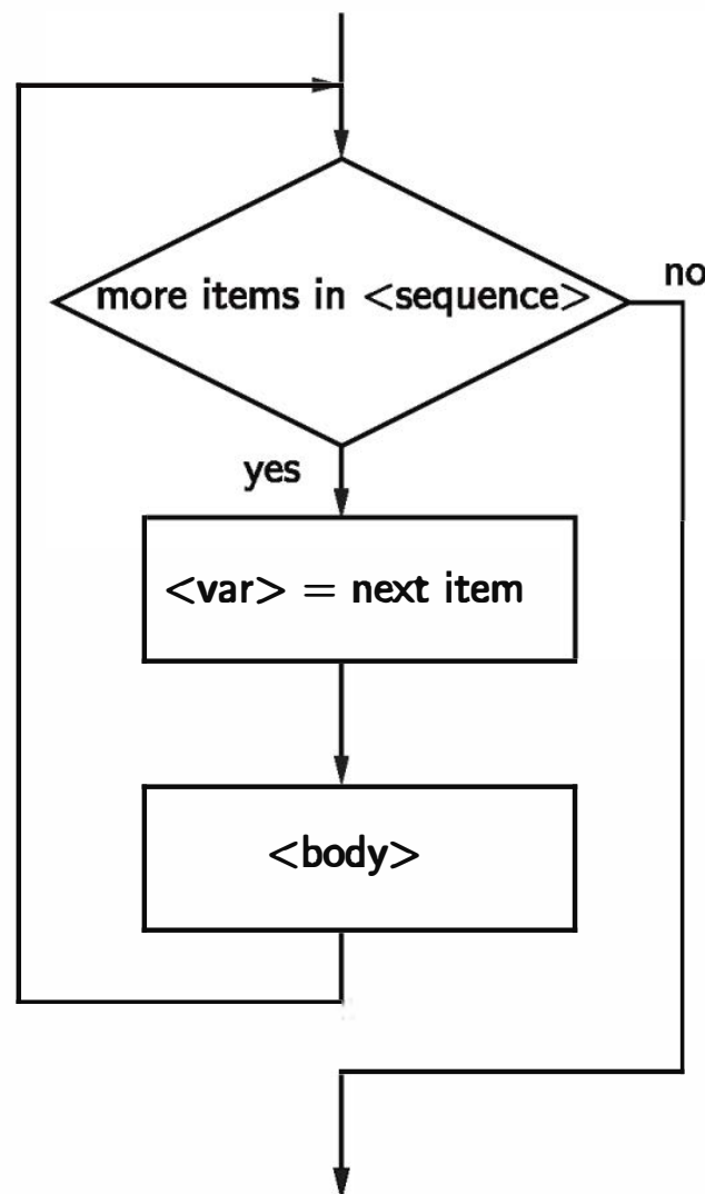
Figure 2.3: Flowchart of a for loop
