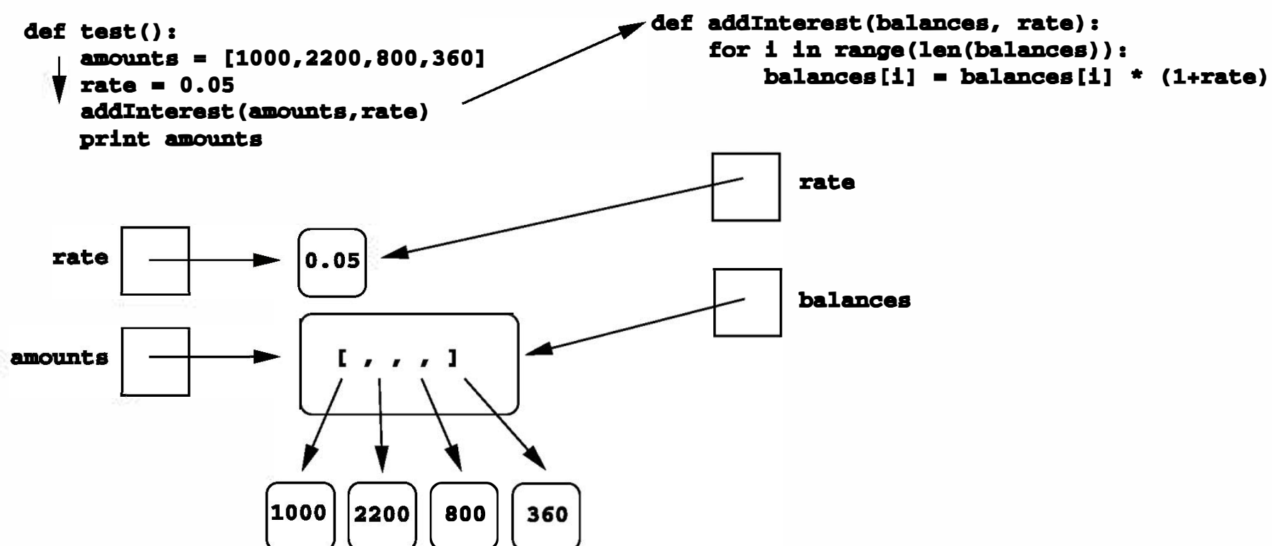
Figure 6.8: Transfer of list parameter to addInterest
