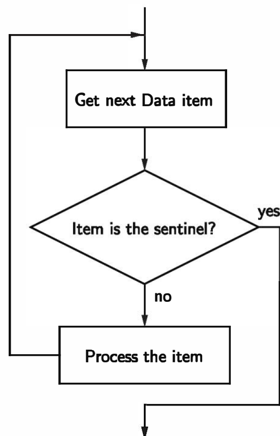
Figure 8.3: Loop-and-a-half implementation of sentinel loop pattern
