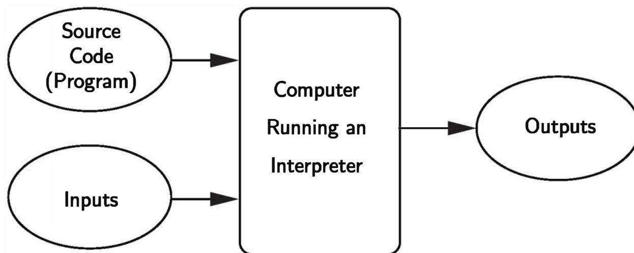
Figure 1.3: Interpreting a high-level language
