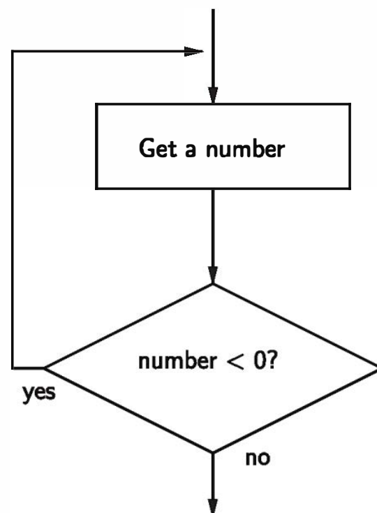
Figure 8.2: Flowchart of a post-test loop
