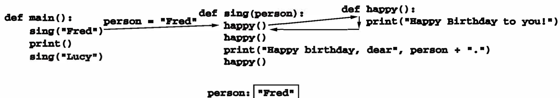
Figure 6.2: Snapshot of completed call to happy
