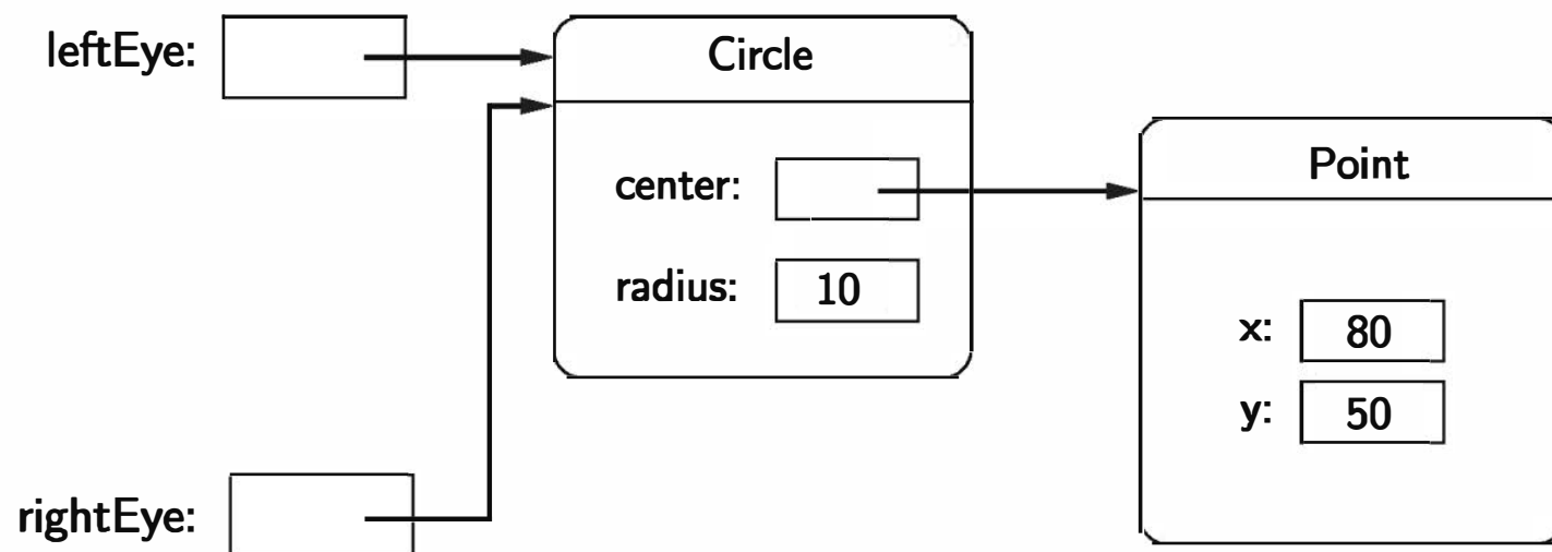
Figure 4.6: Variables leftEye and rightEye are aliases
