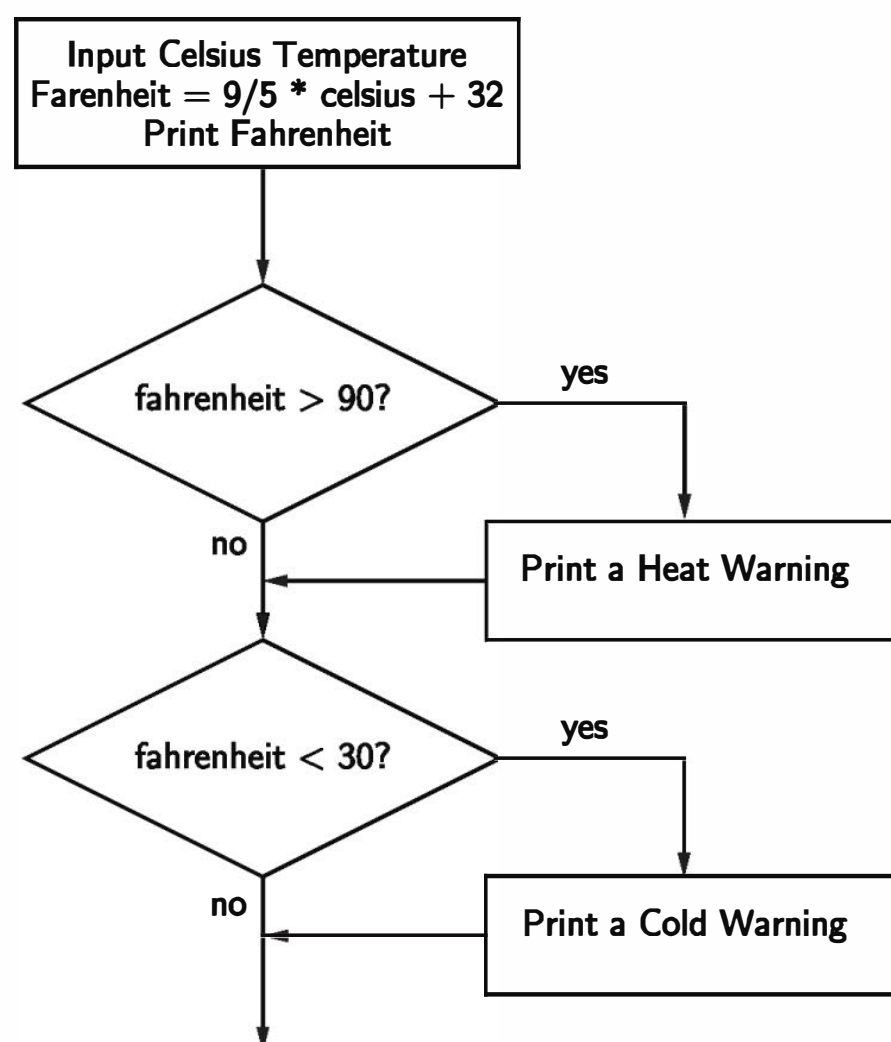
Figure 7.1: Flowchart of temperature conversion program with warnings
