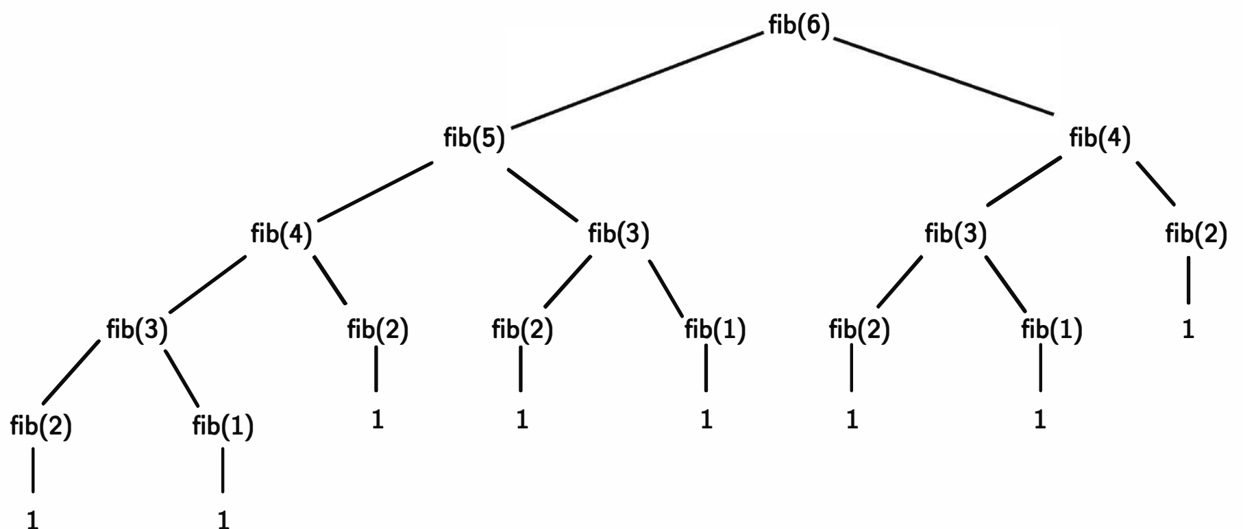
Figure 13.2: Computations performed for fib(6)
