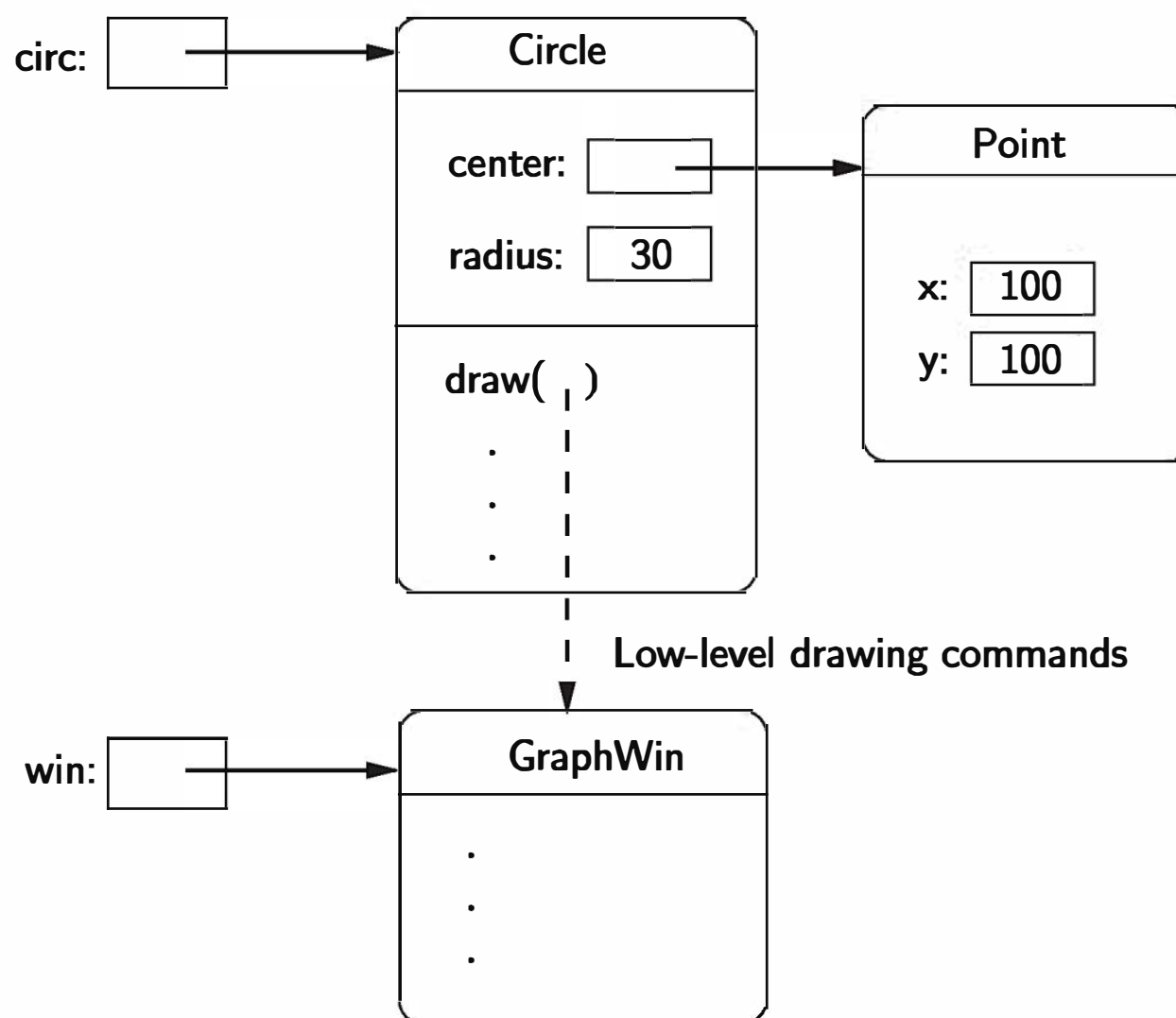
Figure 4.5: Object interactions to draw a circle
