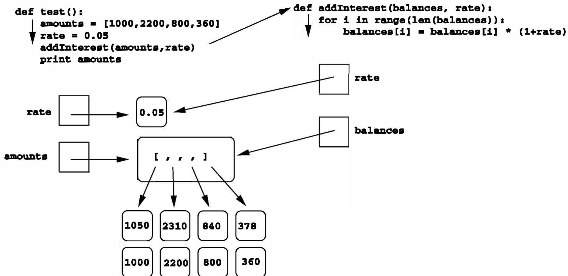
Figure 6.9: List modified in addInterest
