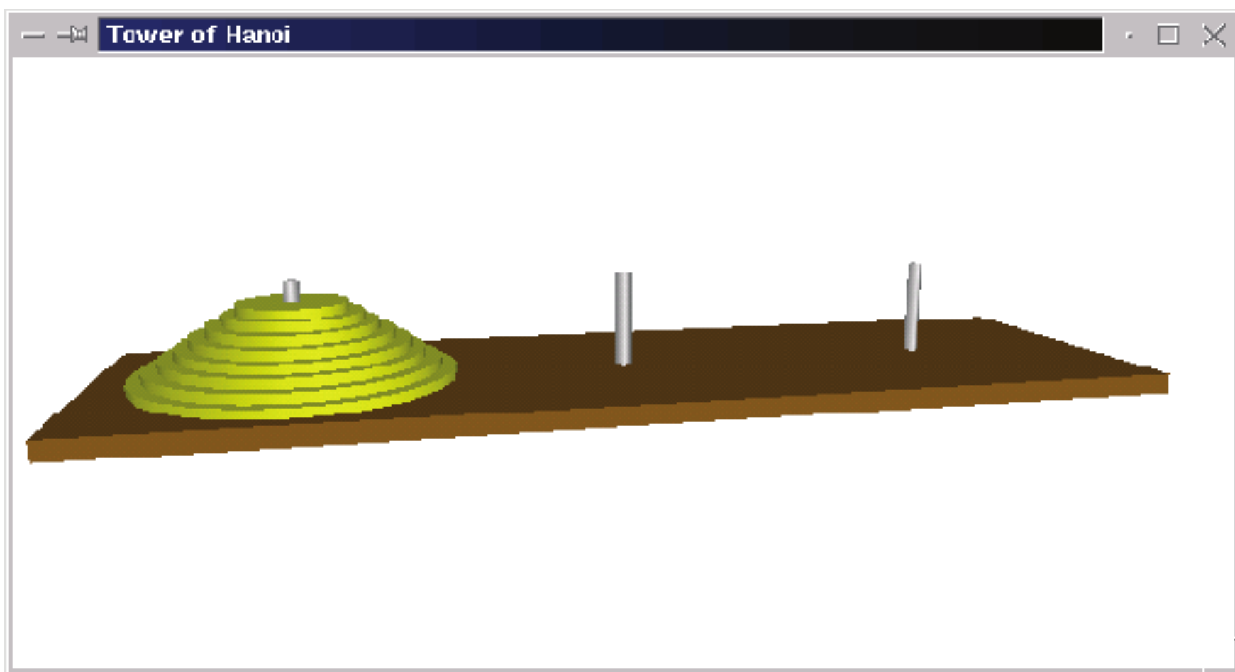
Figure 13.5: Tower of Hanoi puzzle with eight disks
