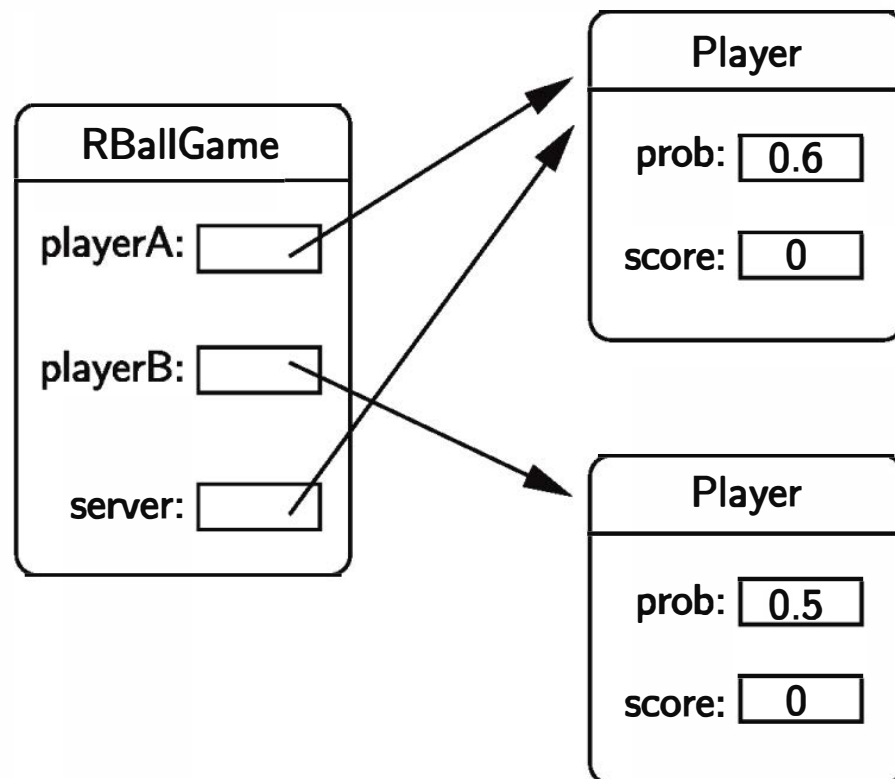
Figure 12.1: Abstract view of RBallGame object
