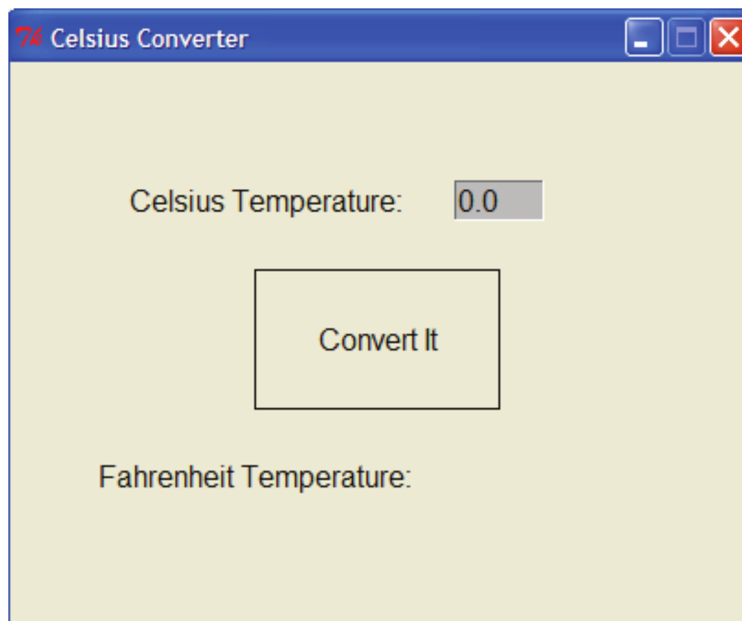
Figure 4.9: Initial screen for graphical temperature converter
