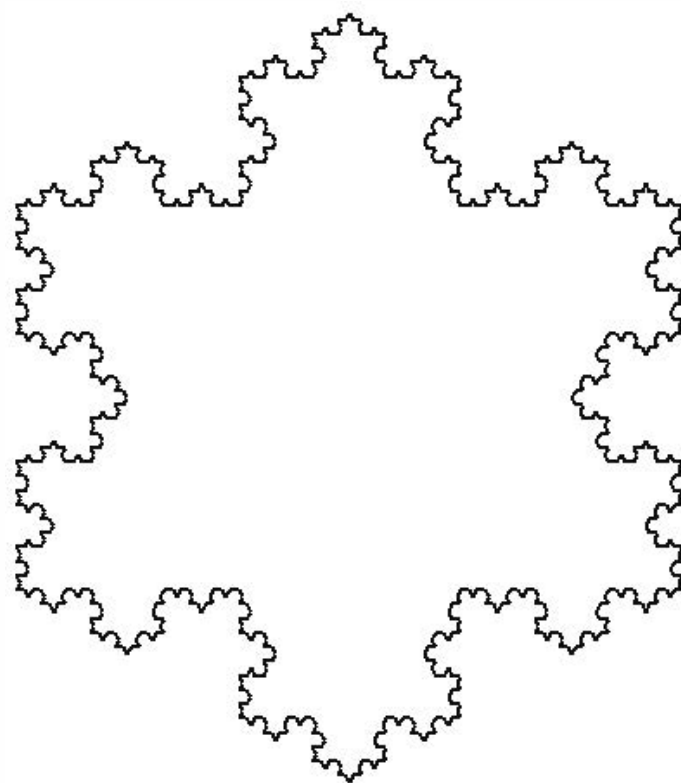
Figure 13.7: Koch snowflake
