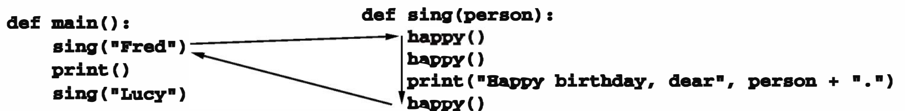
Figure 6.3: Snapshot of completed call to sing
