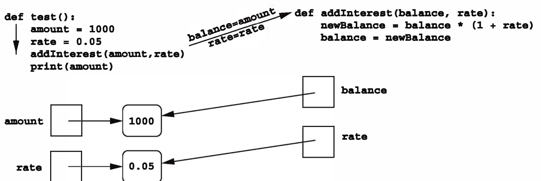
Figure 6.6: Transfer of control to addInterest
