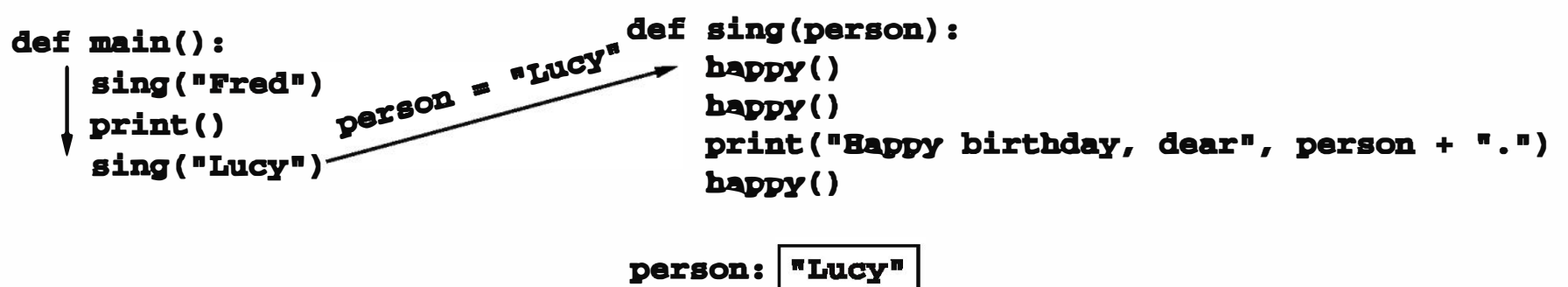
Figure 6.4: Snapshot of second call to sing
