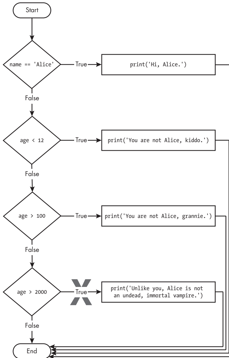
Figure 2-6: The vampire2.py program flowchart. The X path will logically never happen, because if age were greater than 2000, it would have already been greater than 100.
