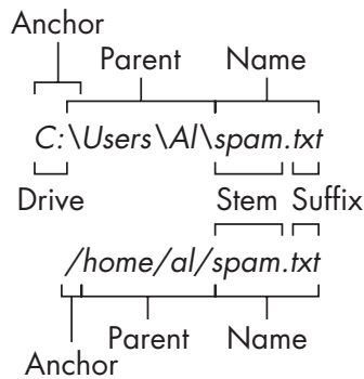
Figure 10-4: The parts of a Windows (top) and macOS/Linux (bottom) filepath
