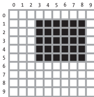
Figure 21-2: The area represented by the box tuple (3, 1, 9, 6)
