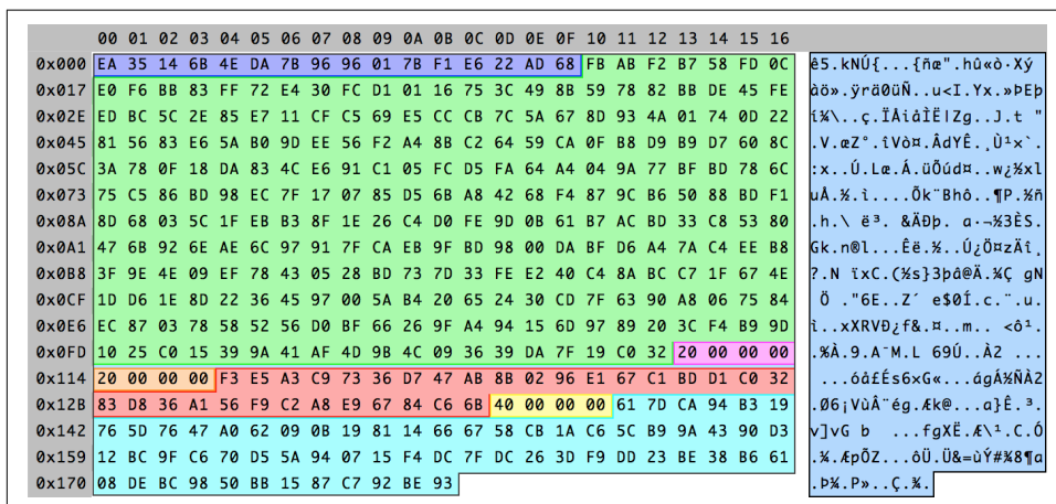
Figure 10-2. Sample of an encrypted CryptoWall file
