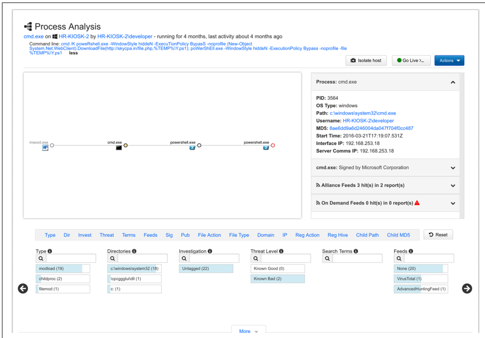
Figure 10-4. Carbon Black blocking PowerWare from executing
