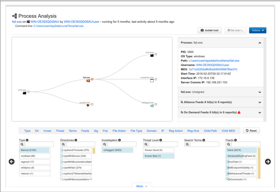
Figure 8-5. Carbon Black blocking Locky’s access to cscript.exe
