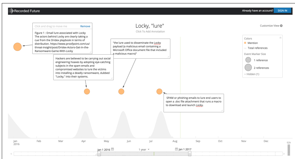
Figure 8-3. Tracking Locky lures in the recorded future portal
