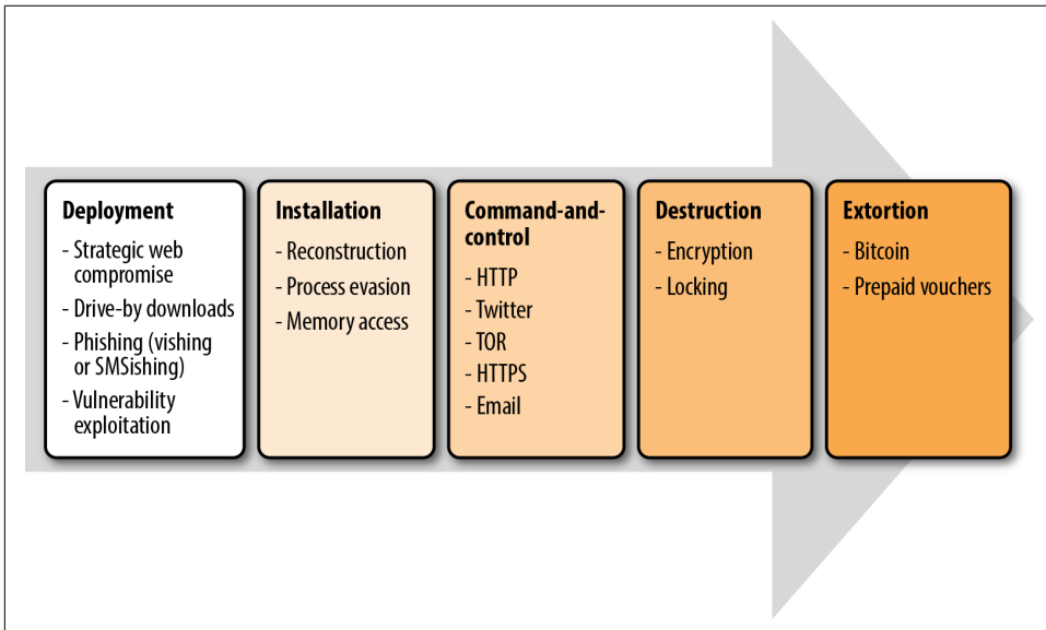
Figure 1-2. Anatomy of a ransomware attack
