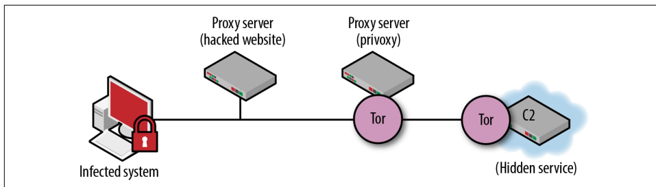
Figure 10-3. CryptoWall 4 communication streams
