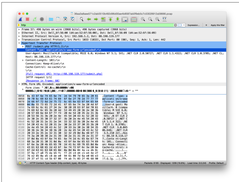
Figure 8-6. Packet capture of Locky traffic
