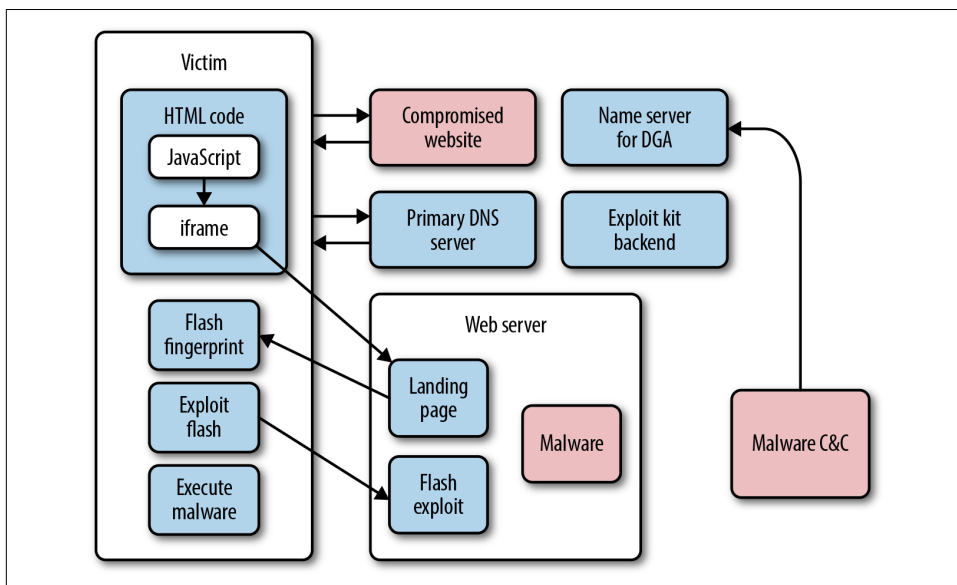
Figure 6-1. An overview of the Neutrino exploit kit
