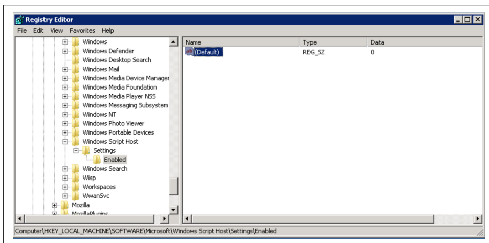
Figure 8-4. Disabling Windows script host
