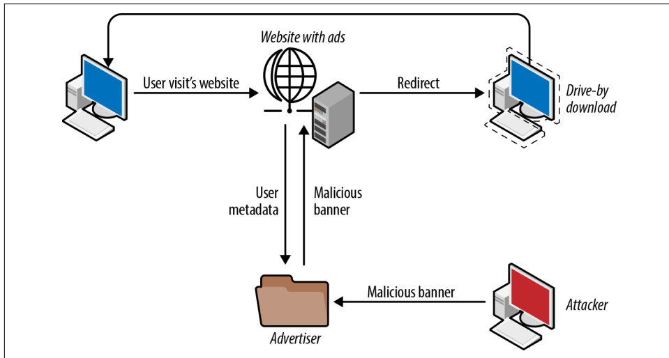
Figure 4-1. How malvertisements work
