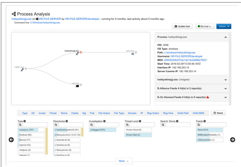
Figure 4-4. Carbon Black stopping TeslaCrypt's attempt to access wmic.exe
