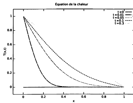
Figure 1.3 - Cloison thermostatée
