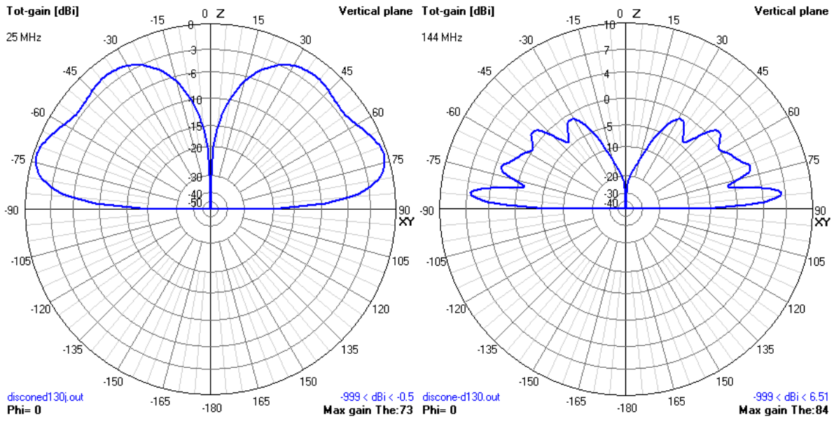
Left: 25 MHz. Right: 144 MHz
