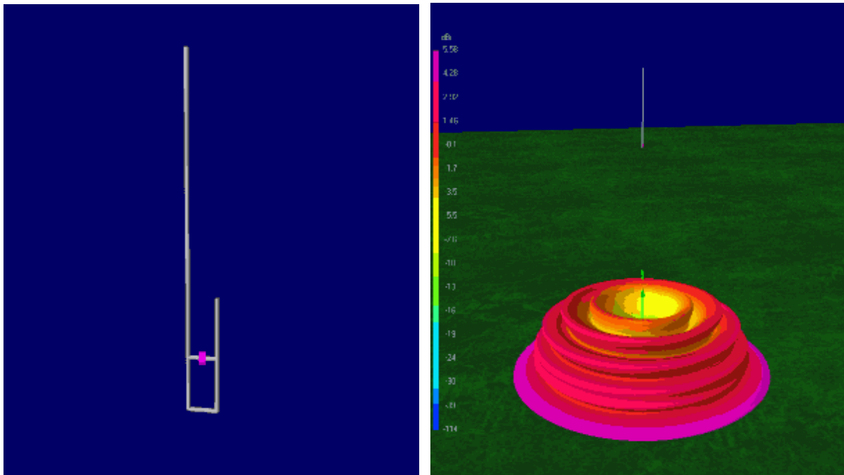
Left: Image of a typical j-pole, Right: 3D Radiation Pattern at 144 MHz and 5m high
