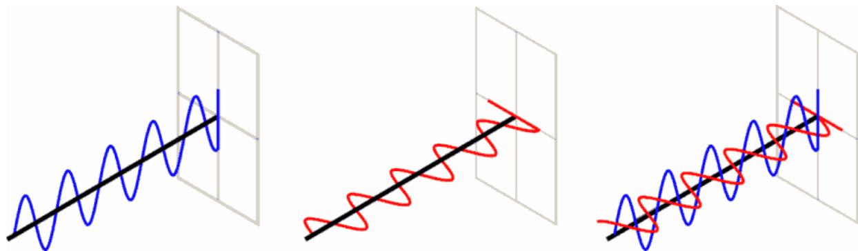
Left: Vertically Polarized, Middle: Horizontally Polarized, Right: Circularly Polarized
