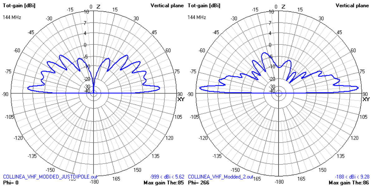
Left: Dipole. Right: One stack.
