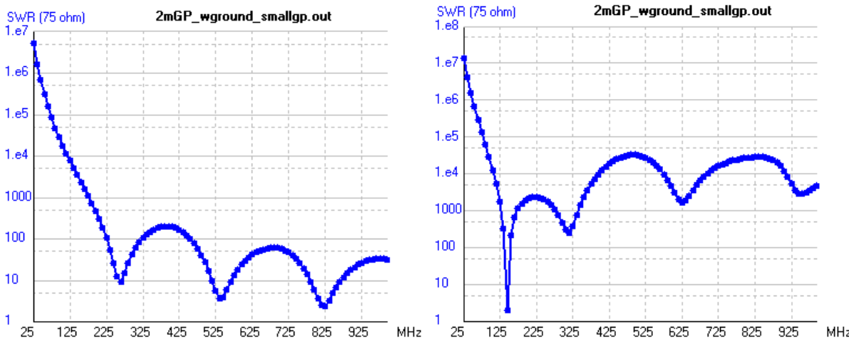
Left: Whip with ground plane of 1cm. Right: Whip with ground plane of 1cm and 2.23 uH loading coil at the base.
