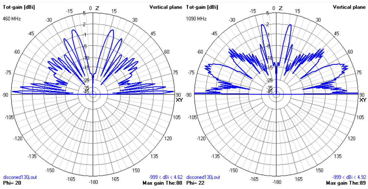
Left: 460 MHz. Right: 1090 MHz
