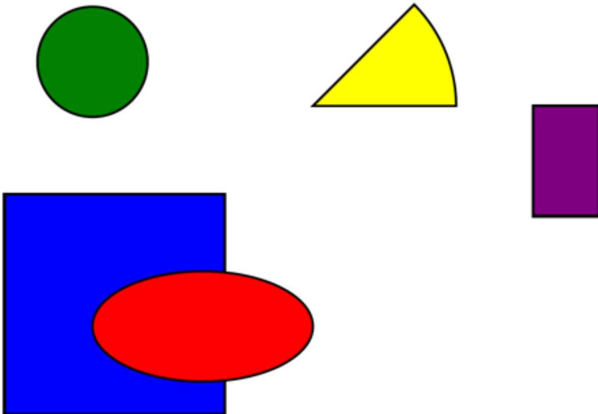
Fig. 9-1: Solid shapes
