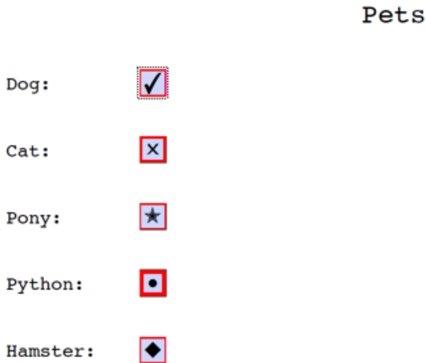
Fig. 10-4: Checked checkboxes
