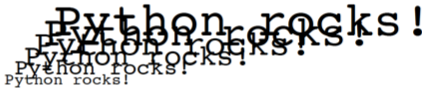
Fig. 9-4: Different strings
