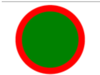
Fig. 9-2: Circle properties
